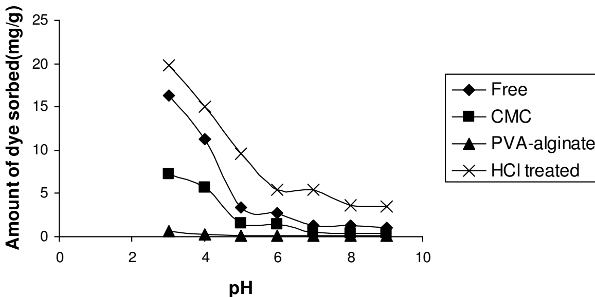
Figure 2. Effect of pH on the biosorption of Direct blue-67 dye (biosorbent dose: 0.1g/50 ml for Direct blue-67, C_0 : 50 mg/l, Temp: 30°C, shaking speed: 100 rpm, particle size: 0.255 mm).
