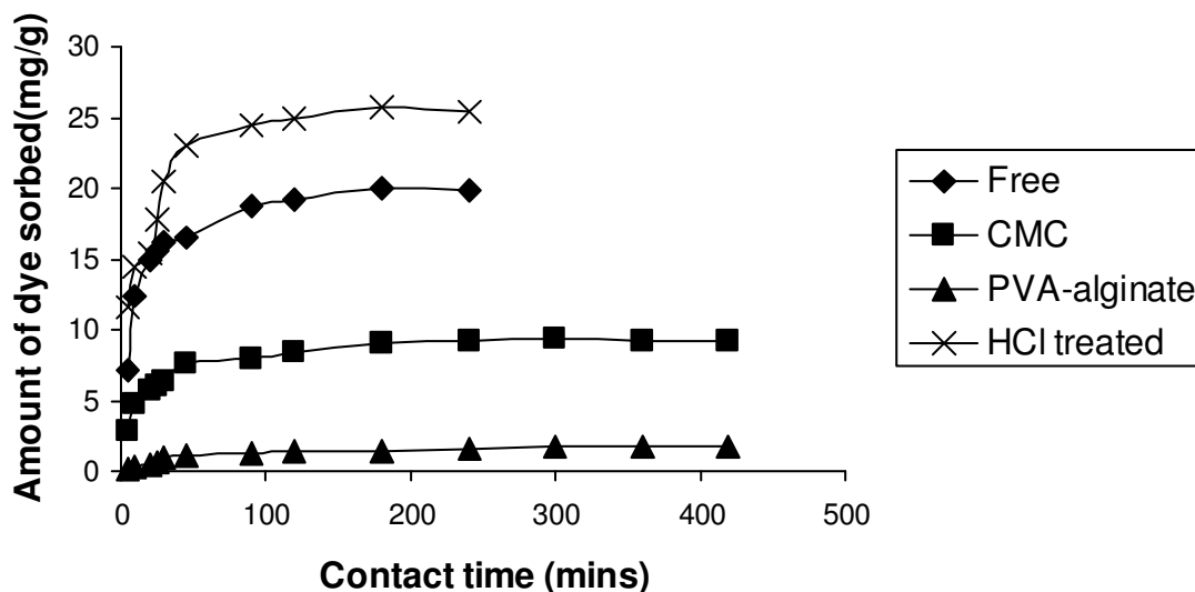
Figure 5. Effect of contact time on the biosorption of Everdirect orange-3GL dye at dye conc, 50 mg/l (biosorbent dose 0.09g/50 ml, Temp: 30°C, shaking speed: 100 rpm, particle size: 0.255 mm, pH: 1).
