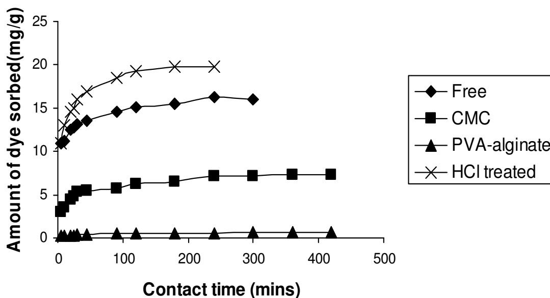
Figure 6. Effect of contact time on the biosorption of Direct blue-67 dye at initial dye conc. 50 mg/l (biosorbent dose 0.1 g/50 ml, Temp: 30°C, shaking speed: 100 rpm, particle size: 0.255 mm, pH: 3).
