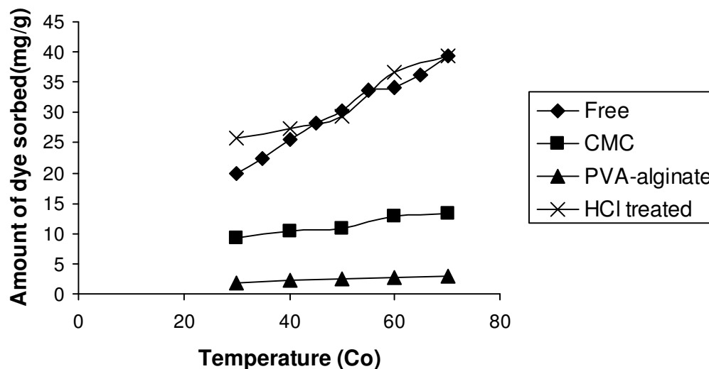
Figure 7. Effect of temperature on the biosorption of Everdirect orange-3GL dye (pH:1, biosorbent dose:0.09 g/50 ml, C_o : 50 mg/l, shaking speed:100 rpm, dyes respectively, particle size: 0.255 mm).
