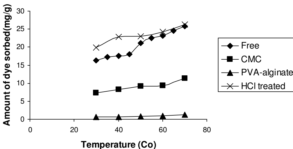
Figure 8. Effect of temperature on the biosorption of Direct blue-67 dyes (pH:1, biosorbent dose: 0.1 g/50 ml for Direct blue-67, C_o : 50 mg/l, shaking speed: 100 rpm, particle size: 0.255 mm).
