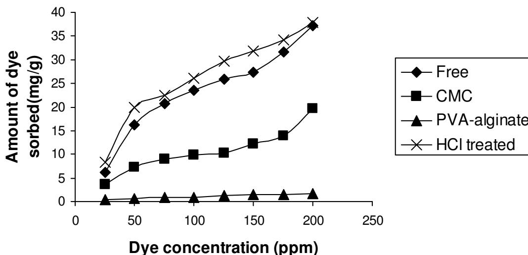
Figure 4. Effect of initial dye concentration on the biosorption of Direct blue-67 dye at biosorbent dose, 0.1g/50 ml ( C_0 : 25, 50, 75, 100, 125, 150, 175 and 200 mg/l, Temp: 30°C, shaking speed: 100 rpm, particle size: 0.255 mm, pH: 3).
