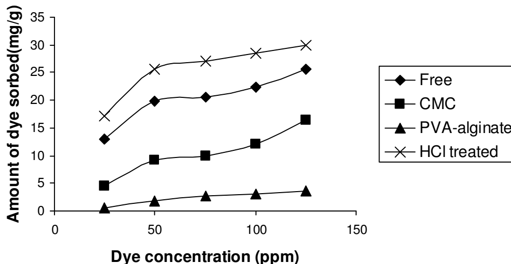
Figure 3. Effect of initial dye concentration on the biosorption of Everdirect orange-3GL dye at t biosorbent dose, 0.1g/50 ml ( C_0 : 25, 50, 75, 100 and 125 mg/l, Temp: 30°C, shaking speed: 100 rpm, particle size: 0.255 mm, pH: 1).
