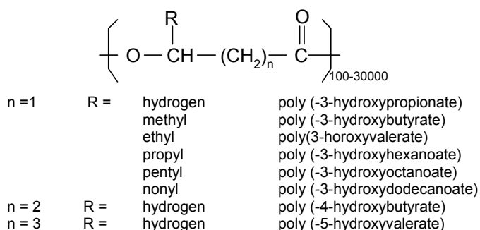
Figure 1. The general structure of polyhydroxyalkanoates.
