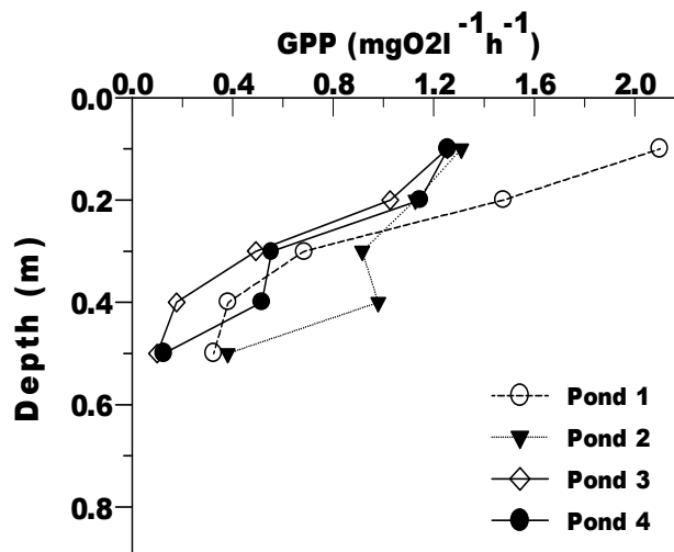
Figure 5. Mean Gross Primary Productivity (GPP) depth profiles of the Walukuba ponds during the sampling time, April to September 2003.
