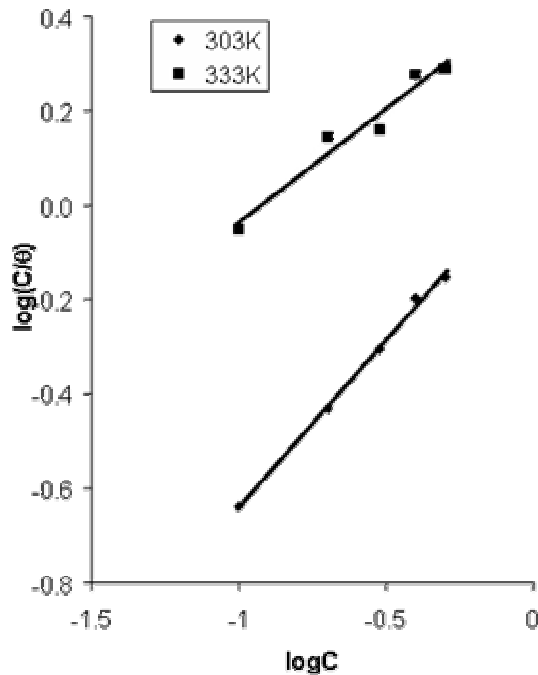
Figure 4. Langmuir isotherm for adsorption of Musa species on the surface of mild steel.
