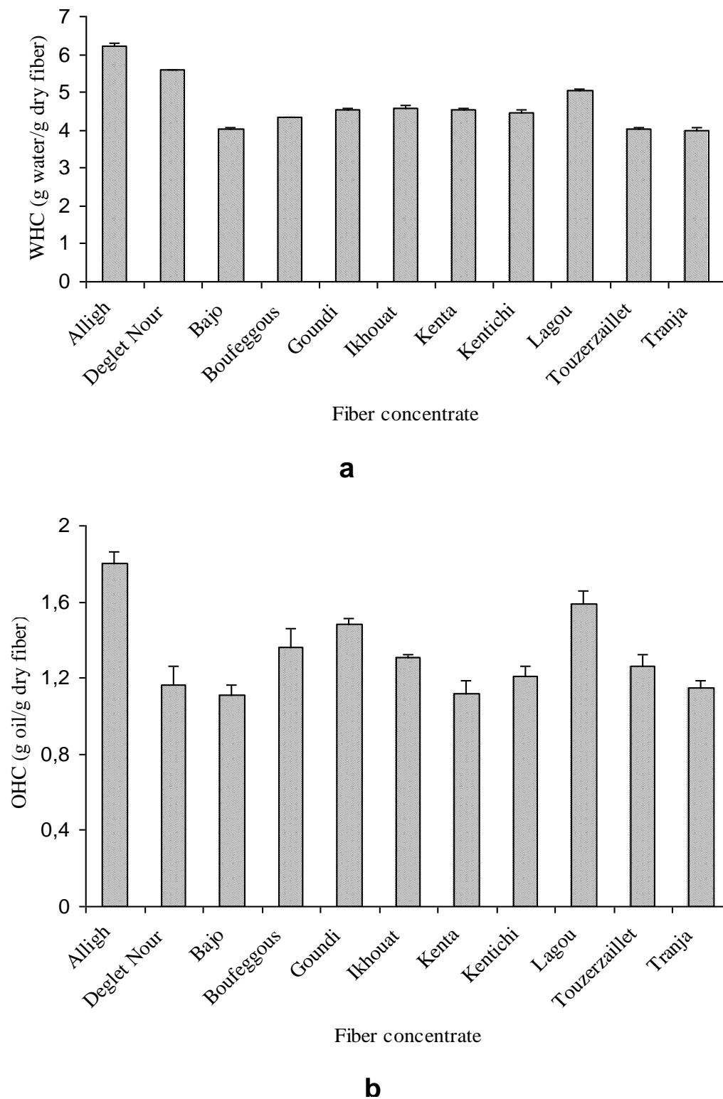
Figure 2. Water holding capacity (a) and oil holding capacity (b) of date fiber concentrates from eleven studied cultivars.
