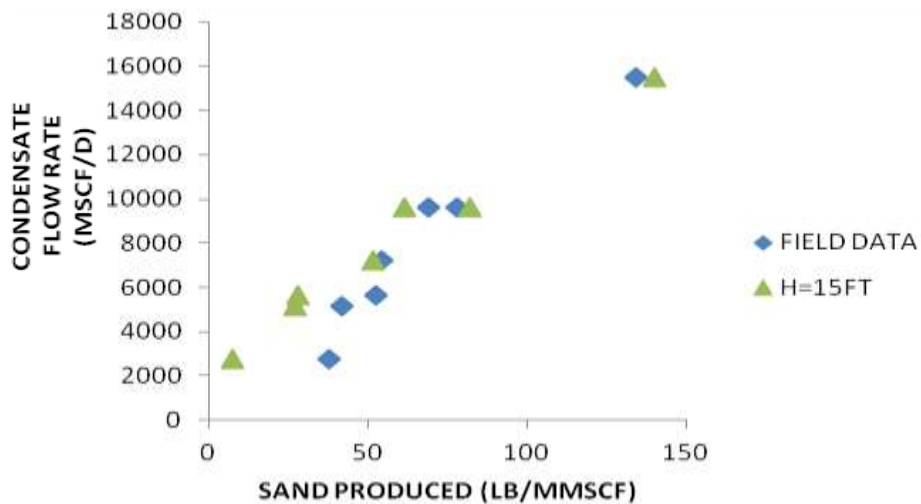
Figure 2. Sand production for Gas Condensate Well 2 at K = 4.3601 \times 10^{-5} .
