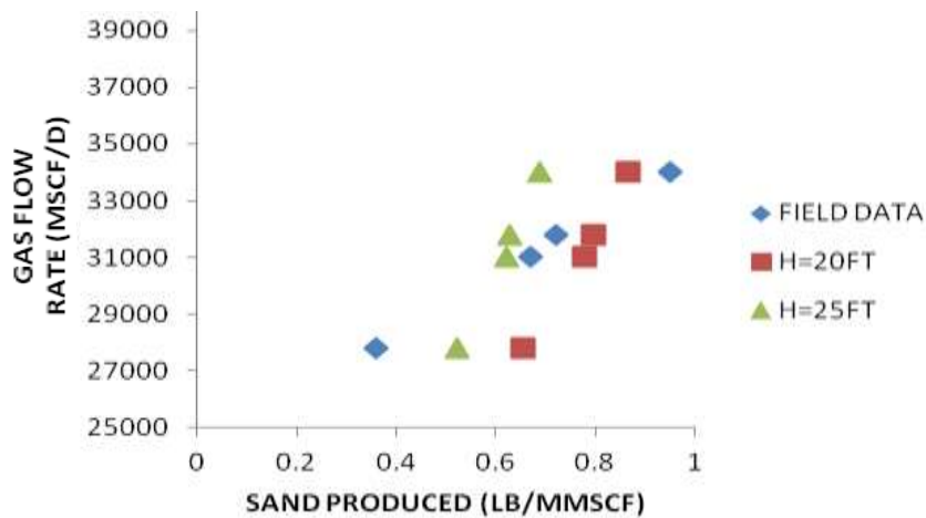
Figure 4. Sand production for Sawan-3 Gas well at K = 8.340 \times 10^{-3} .
