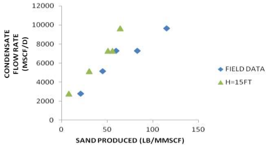
Figure 1. Sand production for gas condensate well 1 at K = 4.1825 \times 10^{-5} .
