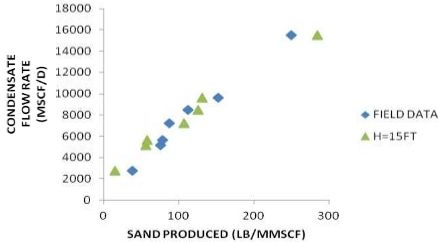
Figure 3. Sand production for condensate well 3 at K = 1.7114 \times 10^{-4} .
