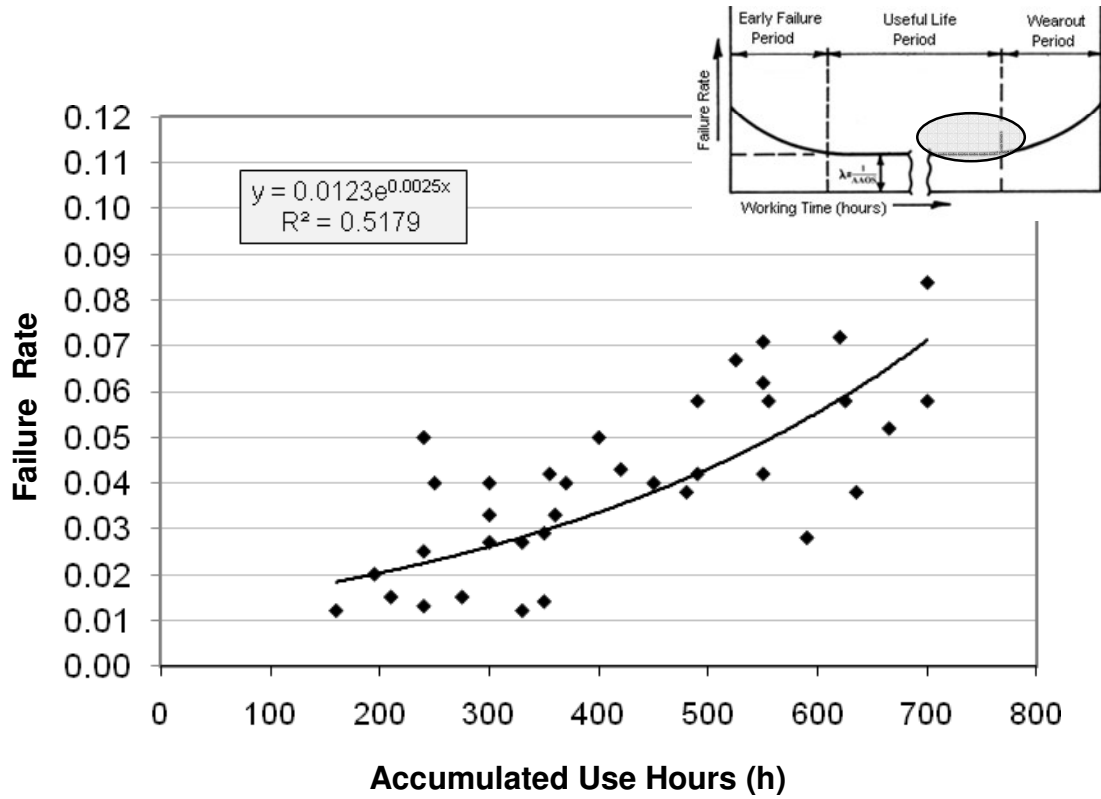
Figure 4. Calculated failure rate vs accumulated use hours for 40 to 80 OAS sub-group.
