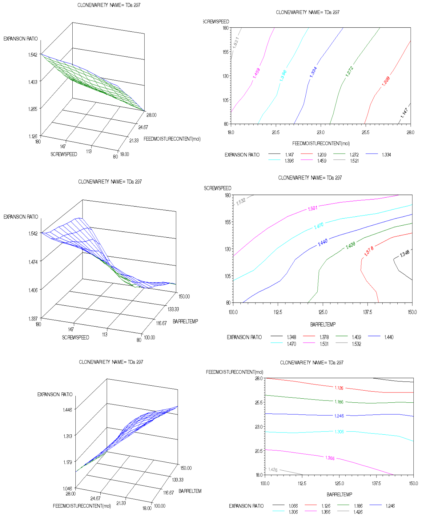
Figure 3. Response surface and contour plots of effect of feed moisture content (%), screw speed (rpm) and barrel temperature (°C) on TDa 297 starch extrudate expansion ratio.
