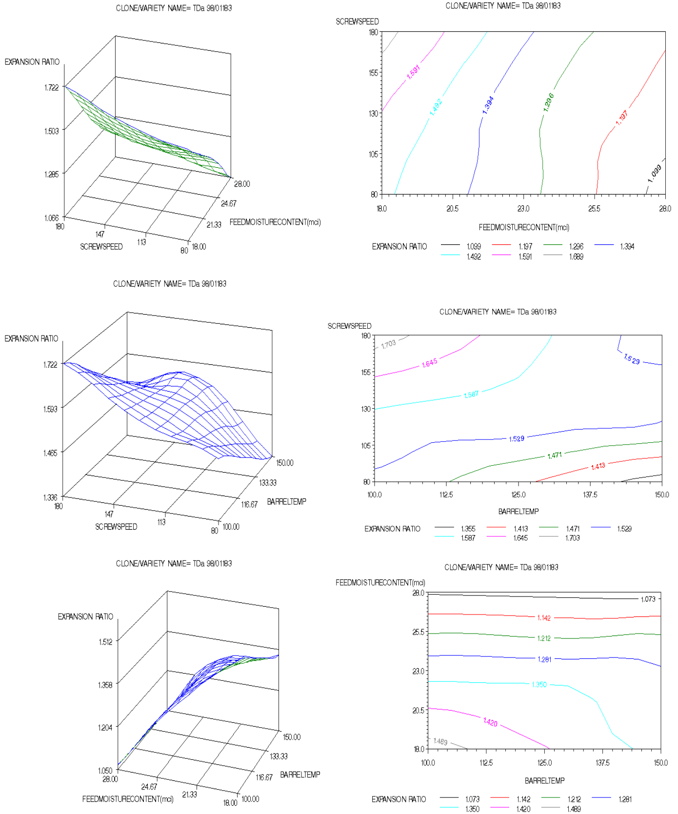
Figure 4. Response surface and contour plots of effect of feed moisture content (%), screw speed (rpm) and barrel temperature (°C) on TDa 98/01183 starch extrudate expansion ratio.
