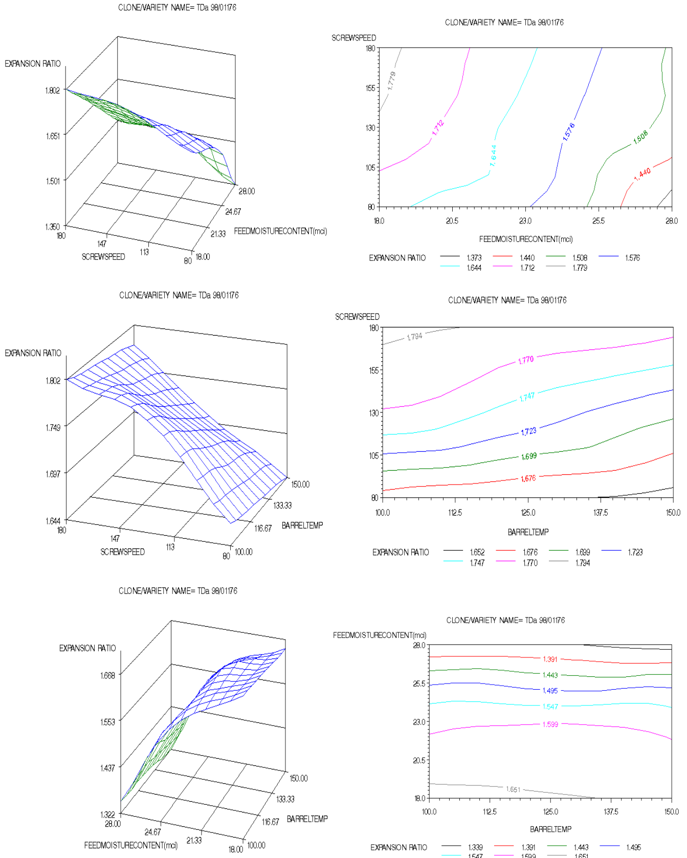
Figure 1. Response surface and contour plots of effect of feed moisture content (%), screw speed (rpm) and barrel temperature (°C) on TDa 98/01176 starch extrudate expansion ratio.
