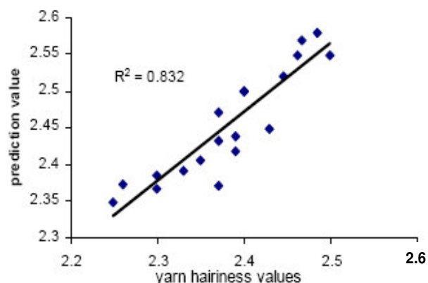
Figure 5. Prediction value versus observed yarn hairiness values.
