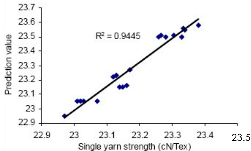
Figure 2. Prediction value versus observe single yarn strength (cN/Tex).
