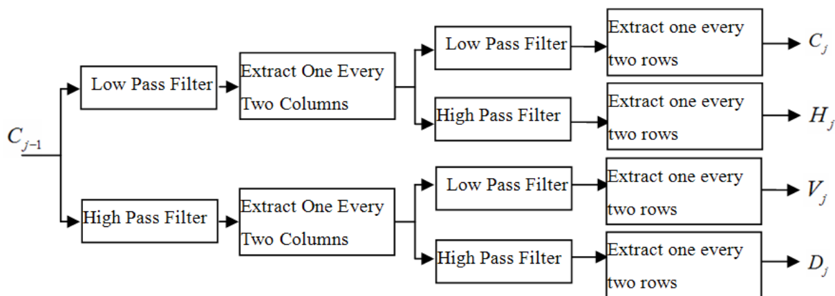
Figure 2. Mallat decomposing flowchart.
