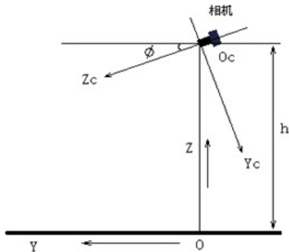
Figure 1. Camera installation and coordinate systems, the right are the combine harvester platform.
