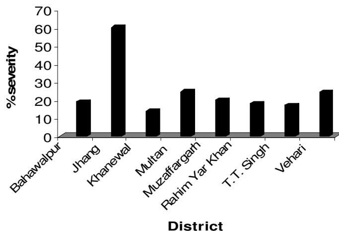
Figure 2. Severity percentage of mango malformation in different mango growing districts of the Punjab Province of Pakistan during the year 2003.
