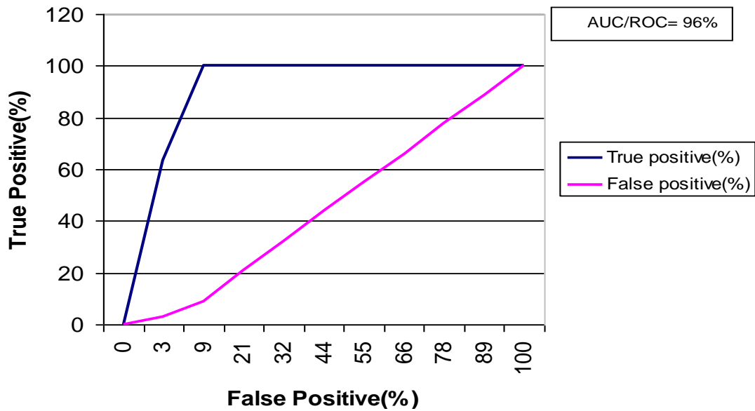
Figure 10. Predictive performance assessment LRM (AUC/ROC).
