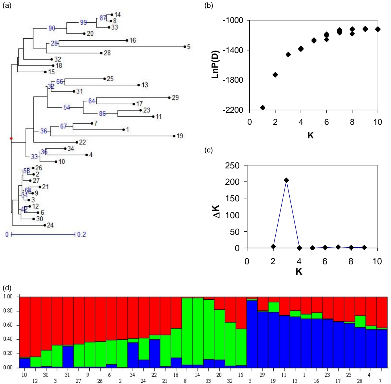
Figure 1. (a) Dendrogram generated by Neighbor joining (NJ) clustering technique showing relationships between 34 genotypes of Salix sp. based on RAPD profiling. Genotypes from 1 to 10 are male; 11 to 30 are half sibs and 31 to 34 are female. Number indicates bootstrap support values. (b) The relationship between the number of cluster (K) and the estimated likelihood of data [LnP(D)]. A model based clustering of 34 genotypes using STRUCTURE without prior knowledge about the populations and under an admixed model calculated that LnP(D) was greatest when K = 3. (c) The relationship between K and \Delta K , that is, \Delta K reaches its maximum when K = 3, suggesting that all genotypes fall into one of the 3 clusters. (d) Grouping of genotypes when K = 3. The genotypes were more likely clustered with respect to one of the 3 clusters. Genotypes from different clusters are represented with different colours: cluster 1 (red), cluster 2 (green) and cluster 3 (blue).
