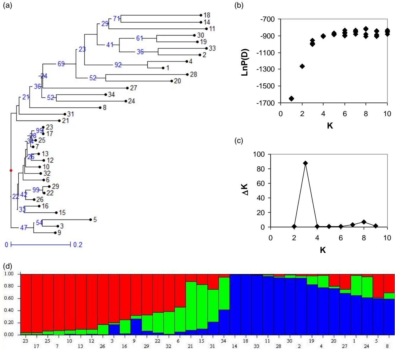
Figure 2. (a) Dendrogram generated by Neighbor joining (NJ) clustering technique showing relationships between 34 genotypes of Salix sp. based on SSR profiling. Genotypes from 1 to 10 are male; 11 to 30 are half sibs and 31 to 34 are female. Number indicates bootstrap support values. (b) The relationship between the number of cluster (K) and the estimated likelihood of data [LnP(D)]. A model based clustering of 34 genotypes using STRUCTURE without prior knowledge about the populations and under an admixed model calculated that LnP(D) was greatest when K = 3. (c) The relationship between K and \Delta K , that is, \Delta K reached its maximum when K = 3, suggesting that all genotypes fell into one of the 3 clusters. (d) Grouping of genotypes when K = 3. The genotypes were more likely clustered with respect to one of the 3 clusters. Genotypes from different clusters are represented with different colours: cluster 1 (red), cluster 2 (green) and cluster 3 (blue).
