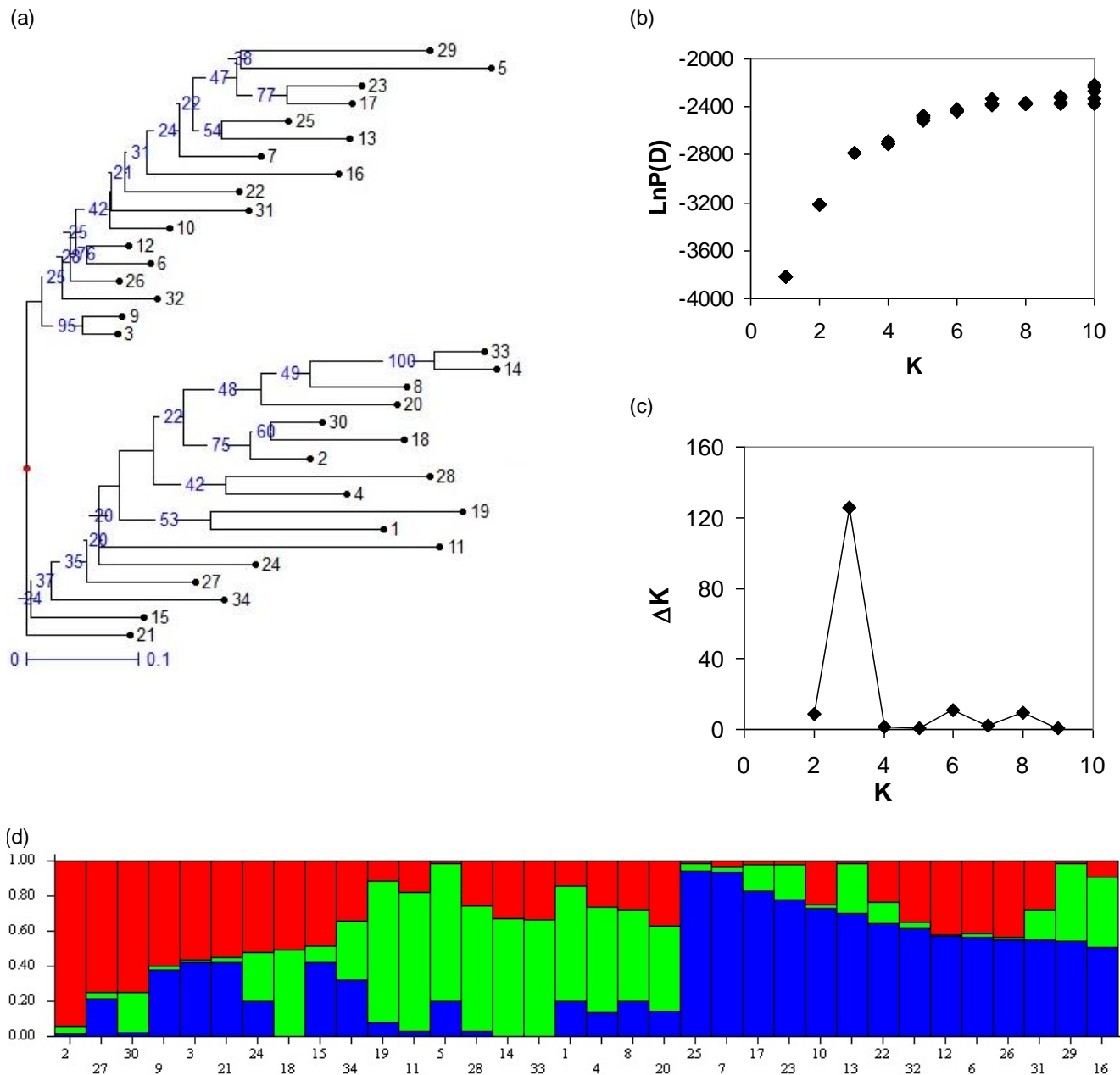
Figure 3. (a) Dendrogram generated by Neighbor joining (NJ) clustering technique showing relationships between 34 genotypes of Salix sp. based on combination of RAPD and SSR profiling. Genotypes from 1 to 10 are male; 11 to 30 are half sibs and 31 to 34 are female. Number indicates bootstrap support values. (b) The relationship between the number of cluster ( K ) and the estimated likelihood of data [ \text{LnP}(D) ]. A model based clustering of 34 genotypes using STRUCTURE without prior knowledge about the populations and under an admixed model calculated that \text{LnP}(D) was greatest when K = 3 . (c) The relationship between K and \Delta K , that is, \Delta K reached its maximum when K = 3 , suggesting that all genotypes fell into one of the 3 clusters. (d) Grouping of genotypes when K = 3 . The genotypes were more likely clustered with respect to one of the 3 clusters. Genotypes from different clusters are represented with different colours: cluster 1 (red), cluster 2 (green) and cluster 3 (blue).
