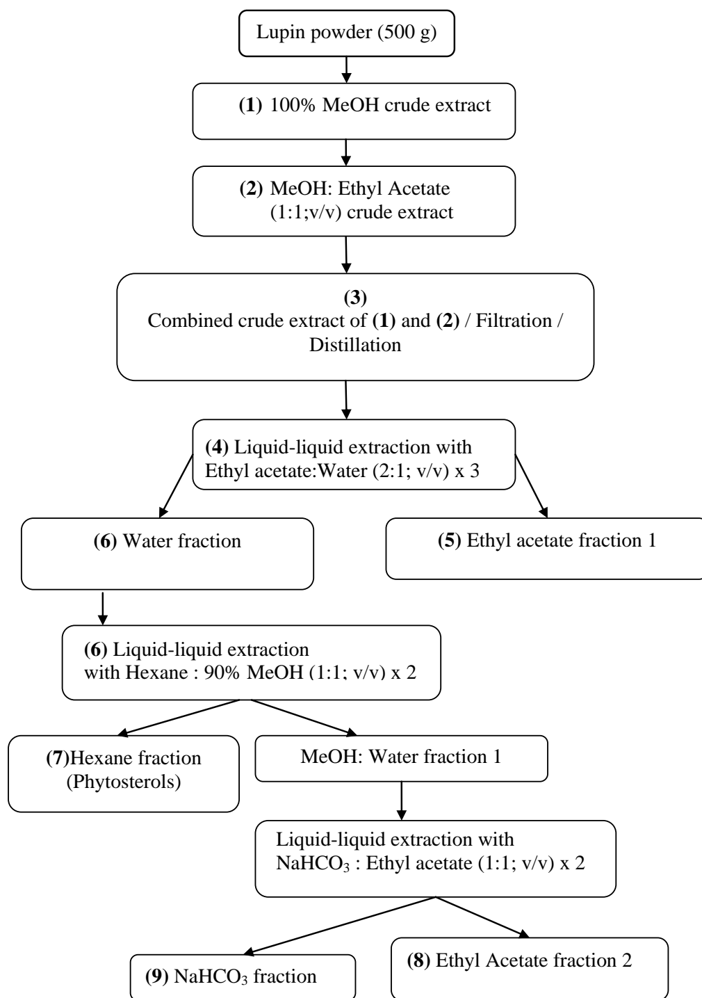
Figure 1. An outline of the procedure followed to extract and fractionate active compounds from Lupinus albus L. seeds (Gamoh et al., 1989).
