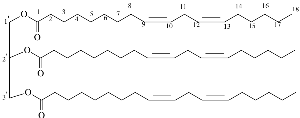
Figure 3. Chemical structure of a bio-stimulatory compound isolated and purified from L. albus seed and identified as C-57 glyceryl trilinoleate ( C_{57}H_{98}O_6 ).
