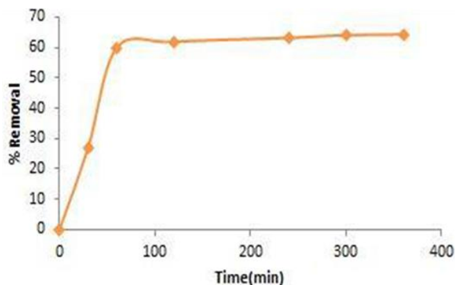
Figure 5. Effect of time over the % removal of \text{Cr}^{+6} .
