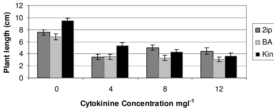
Figure 4. Effect of cytokinine type and concentration on Ficus anastasia length.
