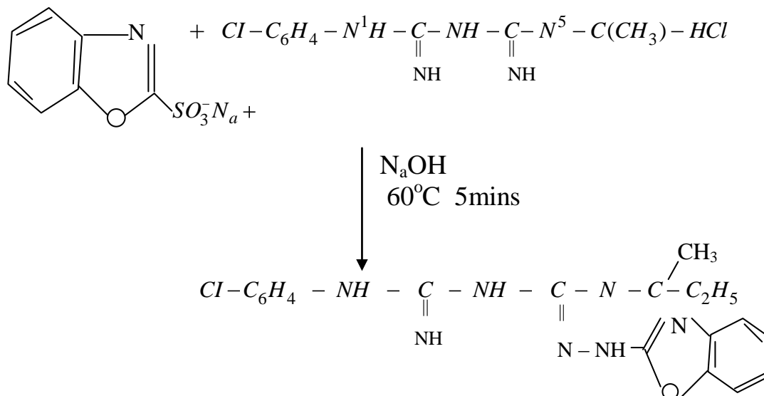
Figure 1. Reaction of sodium benzoxazole-2-sulphonate with proguanil.
