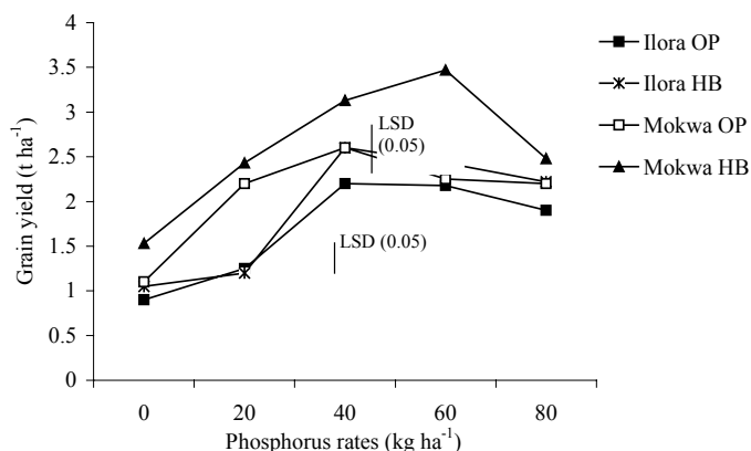
Figure 2. Influence of phosphorus rates on maize yield in the derived and southern guinea savanna zones of Nigeria.
