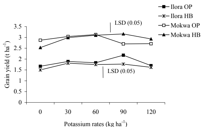
Figure 3. Influence of potassium rates on maize yield in the derived and southern guinea savanna zones of Nigeria.
