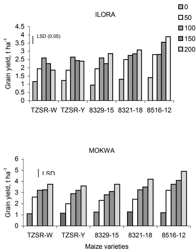
Figure 1. Effect of nitrogen rates (0, 50, 100, 150 and 200 kg ha -1 ) on maize yield in the derived and southern guinea savanna zones of Nigeria.
