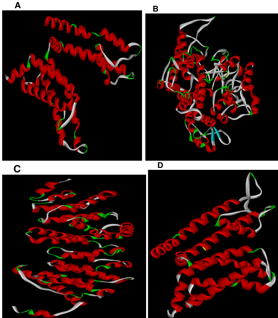
Figure 2. Visualization of CatSper1 (A), CatSper2 (B), CatSper3 (C) and CatSper4 (D) using ViewerLite.
