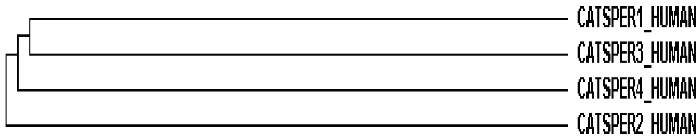
Figure 1. Phylogenetic tree (cladogram) of CatSper protein family using ClustalW.
