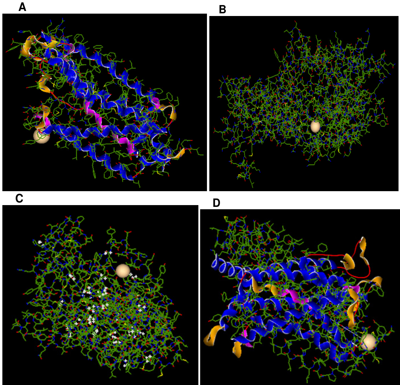
Figure 3. Docking of CatSper1 (A), CatSper2 (B), CatSper3 (C) and CatSper4 (D) with calcium ion.
