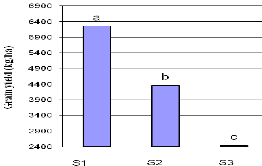
Figure 1. Changes in grain yield under different irrigation levels.
