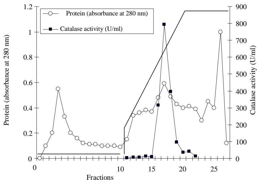
Figure 2. Chromatography of extracellular catalase on DEAE-Sepharose CL 6B. (-o-) Protein; (-■-) extracellular catalase activity; (-) a linear gradient of sodium phosphate buffer using (20 to 500 mM, pH 7).
