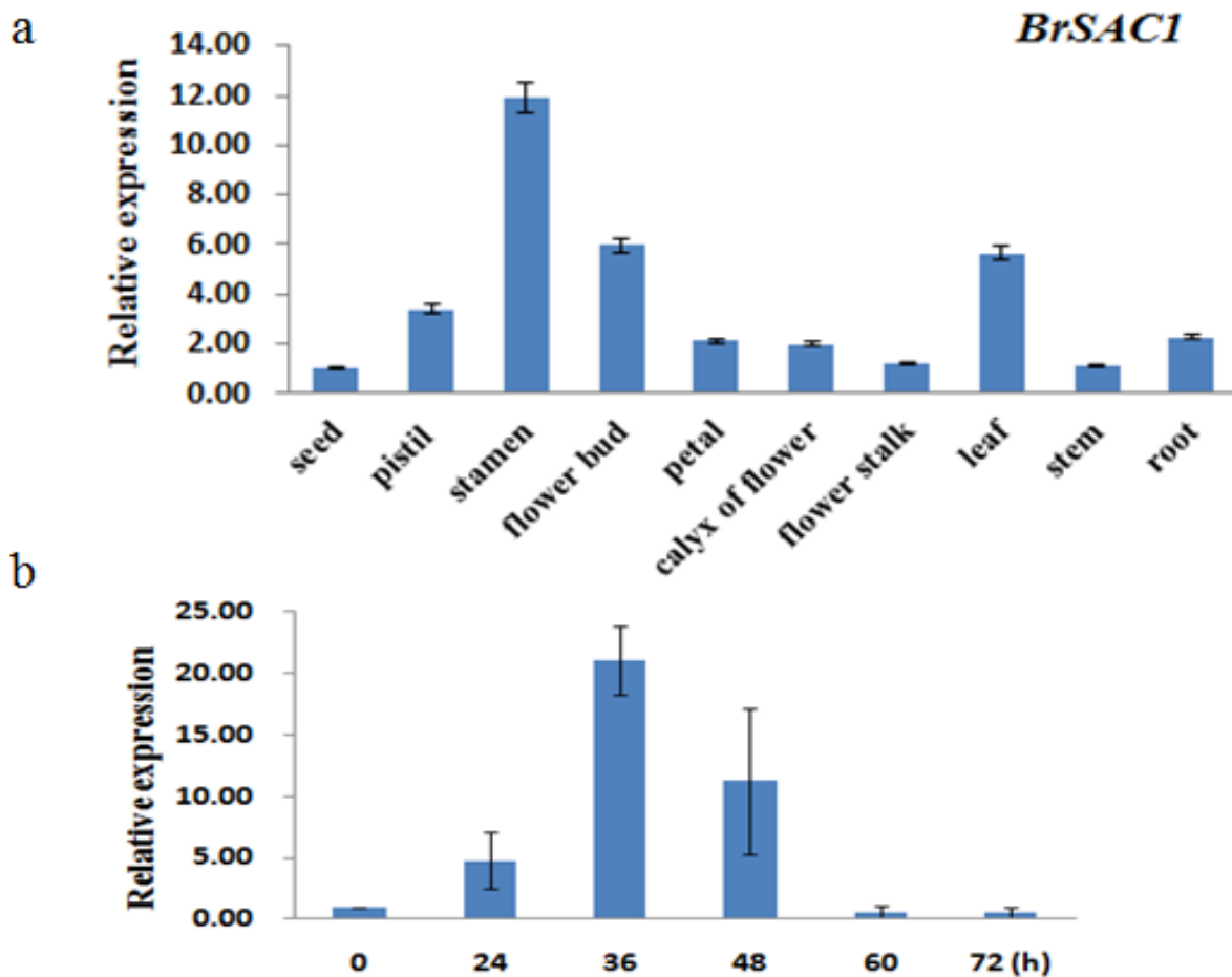
Figure 2. BrSAC1 showing the broad expression across plant tissues using real-time PCR analysis. A. Expression levels of BrSAC1 were measured in various tissues collected from Brassica rapa . B. Real-time PCR analysis of BrSAC1 in germinating seedlings (0-72 h after germination). Amounts of template were calibrated using the mRNA as a reference. Data are presented as means \pm standard deviation of three independently replicated experiments.
