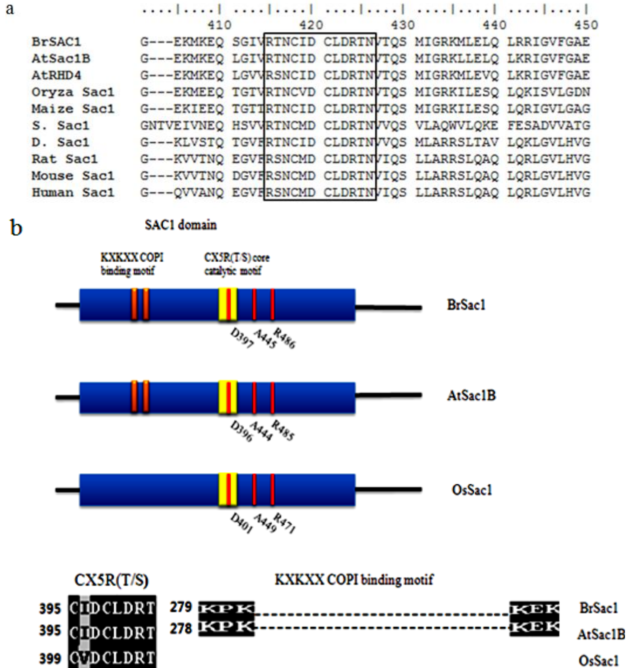
Figure 1. Sequence alignment, domain structure and phylogenetic relationship of BrSAC1 . A. Comparison and deduced amino acid sequence of BrSAC1 and other Sac1 proteins, AtSac1B ( Arabidopsis thaliana ), NP201403; AtRHD4 ( A. thaliana ), NP190714; SAC1 ( Saccharomyces cerevisiae ), CAA82057; Sac1 ( Drosophila melanogaster ), NM138243; rat Sac1 ( Rattus norvegicus ), NP446250; mouse Sac1 ( Mus musculus ), NM030692; human Sac1 ( Homo sapiens ), NM014016; rice Sac1 ( Oryza sativa ), NP001067755; and Maize Sac1 ( Zea mays ), BT086272. Sequence alignment of the core catalytic domains and the KXKXX COPI binding motifs of the SAC1 protein family. The CX 5 R(T/S) core catalytic domain of Sac1 is highly conserved in yeast, higher plants, Drosophila , and mammals. Identical and conserved residues in all aligned sequences are indicated by the rectangle box. B. (a) Diagrams of the domain organization of Sac1 proteins. Domains and motifs of interest are highlighted by colored boxes. Blue boxes show the Sac1-catalytic domain, yellow boxes show the CX 5 R(T/S) core catalytic motif, and orange boxes show the KXKXX COPI binding motif. Three key amino acids within the Sac1 domain known to affect catalytic activity (Rivas et al., 1999; Liu et al., 2008) are indicated in red. (b) Sequence alignment of the core catalytic domains and the KXKXX COPI binding motifs of the Sac1 protein families. Identical amino acids are highlighted by black boxes. C. The phylogenetic tree of the Sac1 protein family. BrSAC1 isolated in this study. A phylogenetic tree was constructed using CLC Main workbench 5 with CLUSTAL W alignments as input using the neighbor-joining method (Saitou and Nei 1987) to construct the tree.
