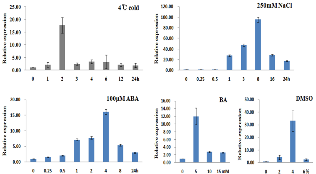
Figure 3. BrSAC1 expression is induced by abiotic stress treatments in Brassica seedlings. Expression levels were examined by RT-PCR at various times after treatment with cold (4°C), salt (250 mM NaCl), or 100 µM abscisic acid (ABA). Expression profiles were also examined in the presence of various concentrations of chemical modulators of membrane fluidity benzyl alcohol (BA) at 4°C and DMSO at room temperature. Actin was used as a positive control and to determine relative expression for each treatment.
