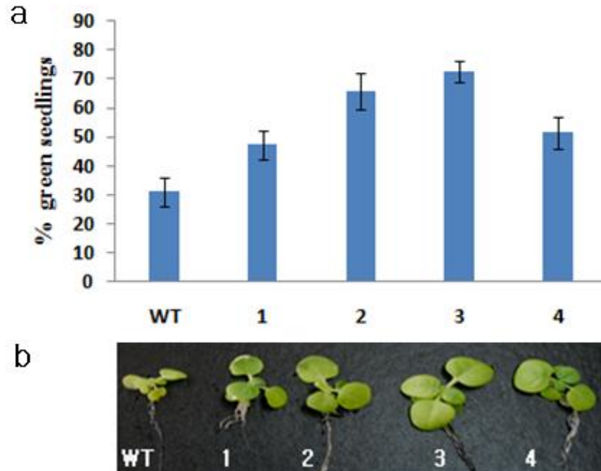
Figure 5. Plants overexpressing BrSAC1 showed increased salt tolerance. Seedlings of tobacco seedlings from transgenic lines (1 to 4) overexpressing BrSAC1 were examined for effects of salt treatment. A. The number of non-chlorotic (Green) 21 day old seedlings (WT and transgenic lines) were counted following a 4 day 250 mM NaCl salt-stress treatment and eight day recovery period. B. Pictures of representative seedlings from (A) are shown at the end of the recovery period.
