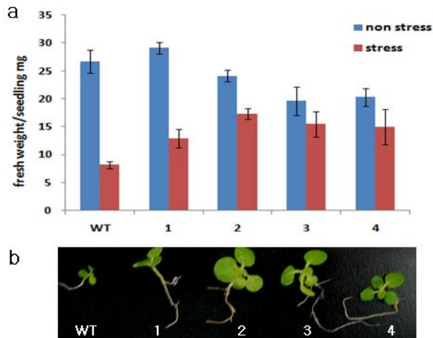
Figure 6. Plants overexpressing BrSAC1 showing increased cold tolerance. Tobacco seedlings from transgenic lines (1 to 4) overexpressing BrSAC1 were examined for effects of cold stress: A. Fresh weight of 21-day-old seedlings (WT and transgenic lines) that were cold-stressed (4°C) for 15 days, followed by a 15 day recovery, was measured for comparison with that of unstressed controls. B. Pictures of representative seedlings from (A) at the end of the recovery period.
