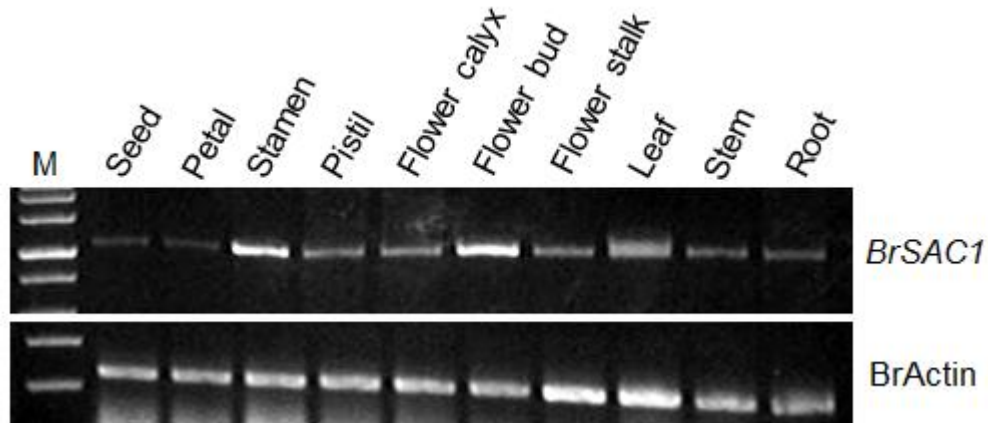
Supplemental Figure 1 for Figure 2. Han et al. BrSAC1 showing broad expression across plant tissues. Semi-quantitative reverse transcription-polymerase chain reaction (RT-PCR) analysis of BrZFP1 was conducted in various tissues collected from Brassica rapa . Actin was used as a positive control and was detected in all tissues shown as the set of lower bands.
