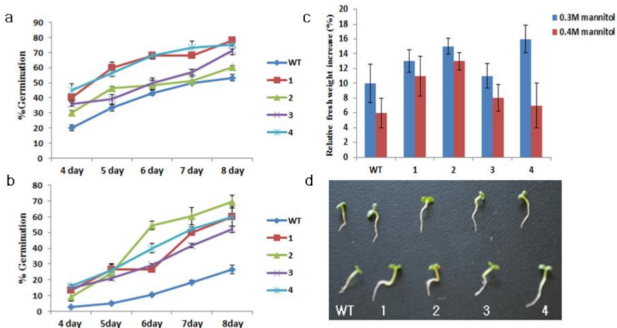
Figure 7. Plants overexpressing BrSAC1 showing increased dehydration tolerance. Tobacco seedlings overexpressing BrSAC1 (transgenic lines 1 to 4) were examined for effects of dehydration stress. Percent germination of seeds (WT and transgenic lines) sown on 0.3 M (A) and 0.4 M (B) mannitol is shown for four to eight days after the start of germination. (C) Percent increase in relative fresh weight (FW) of 8-day-old seedlings germinated on 0.3 M or 0.4 M mannitol is shown relative to the FW of unstressed seedlings. (D) Pictures of representative seedlings of WT and transgenic lines taken 8 days after germination on 0.3 M (upper) and 0.4 M (lower) mannitol.
