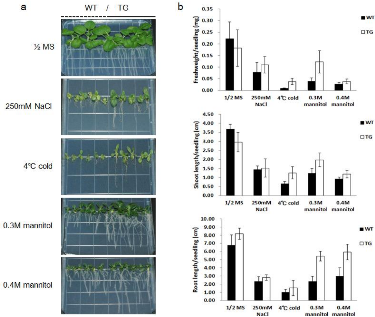
Figure 4. Plants overexpressing BrSAC1 showing enhanced tolerance to stress. Tobacco plants overexpressing BrSAC1 (transgenic lines: TG) and WT plants were examined under various stress conditions. The 10-day-old seedlings grown on 1/2 MS medium were transferred to new media containing 250 mM NaCl for salt stress, 0.3 M or 0.4 M mannitol for dehydration stress, or placed at 4°C for cold stress. After 18 days of stress treatment, plants were photographed (A) and examined for relative fresh weight and shoot and root lengths. Data are represented as average \pm standard deviation for 5 plants from 1 representative experiment (B). In this analysis, significant P values of 0.015 to 0.02 (FW), 0.015 to 0.02 (shoot lengths), and 0.02 to 0.025 (root lengths) were obtained between WT and transgenic lines (TG1 and TG2).
