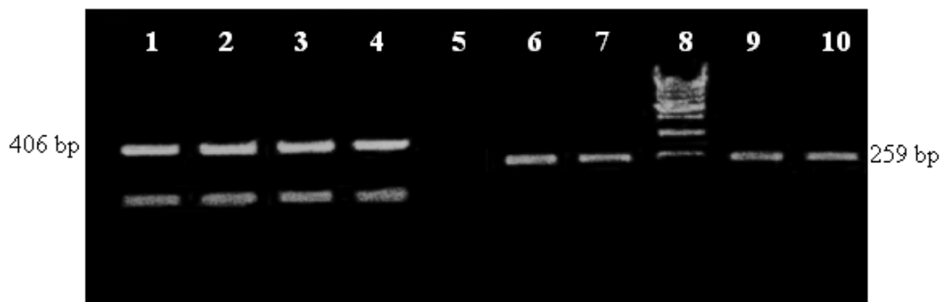
Figure 1. Agarose gel electrophoresis showing the amplification of 406 bp fragments of E. coli serovar O111 (lanes 1, 2, 3, 4) and amplification of 259 bp fragment of E. coli serovar O157:H7 (lanes 6, 7, 9, 10). Lane 8 shows 250 bp ladder.
