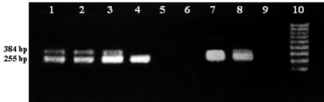
Figure 2. Agarose gel electrophoresis showing amplification of 384 and 255 bp fragments of intimin and shiga toxin type two genes of E. coli serovar O157:H7, respectively (lanes 1, 2 and 3). While lanes 7 and 8 show 255 bp fragments of shiga toxin type two gene only. Lane 10 shows 100 bp ladder.
