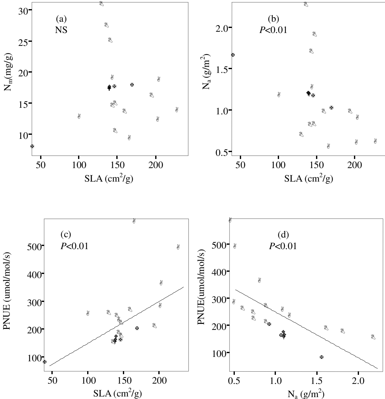
Figure 2. Relationships among the specific leaf areas, nitrogen contents ( N_m and N_a ) and photosynthetic nitrogen use efficiency of the dominant species. The different markers stand for different species. The open circle stands for the herb community, the open triangle stands for the shrub community, the solid triangle stands for the early forest community and the solid circle stands for the climax forest community.
