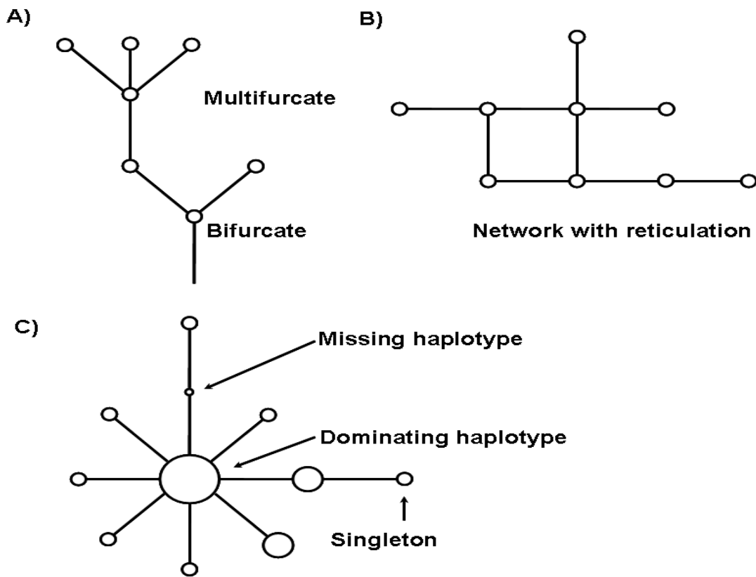
Figure 2. A) The traditional way of describing evolutionary relations between taxa is a furcating tree. B) Phylogenetics networks can display relations enhanced by a phylogenetic tree. Different parts of an information source (for example, gene or alignment part) can squabble for a different topology visualized by a loop or a cycle. C) Star-like structure of a minimum spanning network shows a numerical dominating central haplotype surrounded by several haplotypes (high haplotypes diversity), which show little differences (low nucleotide diversity). This pattern suggests that most haplotypes originate recently and is indicative of a population expansion during the recent history of the taxa, as well as, the event of the initial effect that can be hypothesized.
