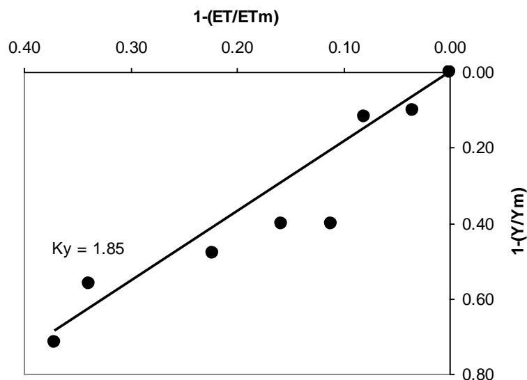
Figure 2. Relative yield decrease of cotton as a function of relative ET deficiency.
