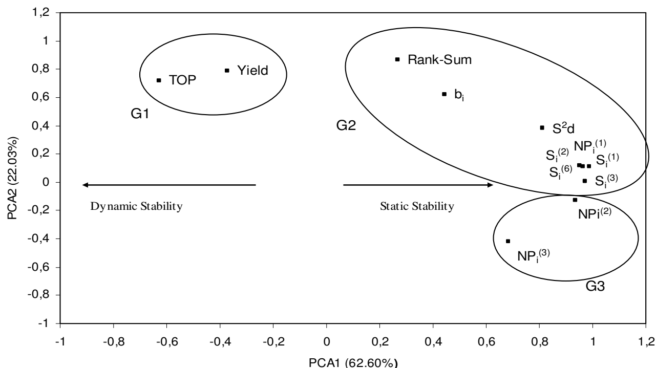
Figure 1. Principal component analysis (PCA1 and PCA2) plot of ranks of stability of yield, as estimated with 11 methods based on yield data from 8 barley cultivars grown in 11 environments, showing the interrelationships between these parameters.
