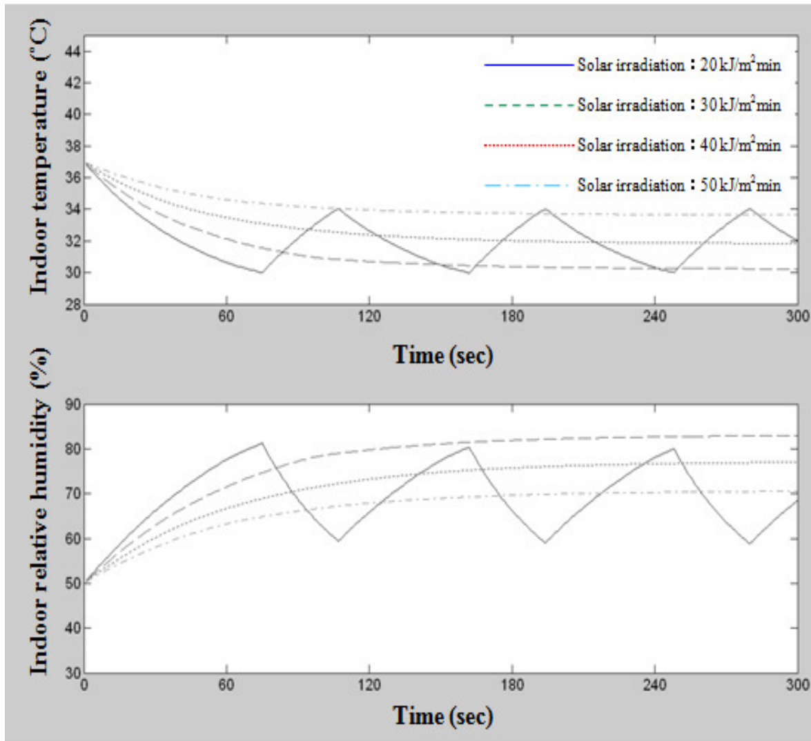
Figure 4. Variation of the inside temperature and relative humidity (spray on : 34°C d.b.; off : 30°C d.b.).
