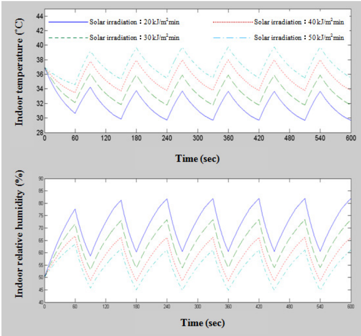
Figure 7. Variation of the inside temperature and relative humidity (fogging on: 1 min and interval: 30 s).
