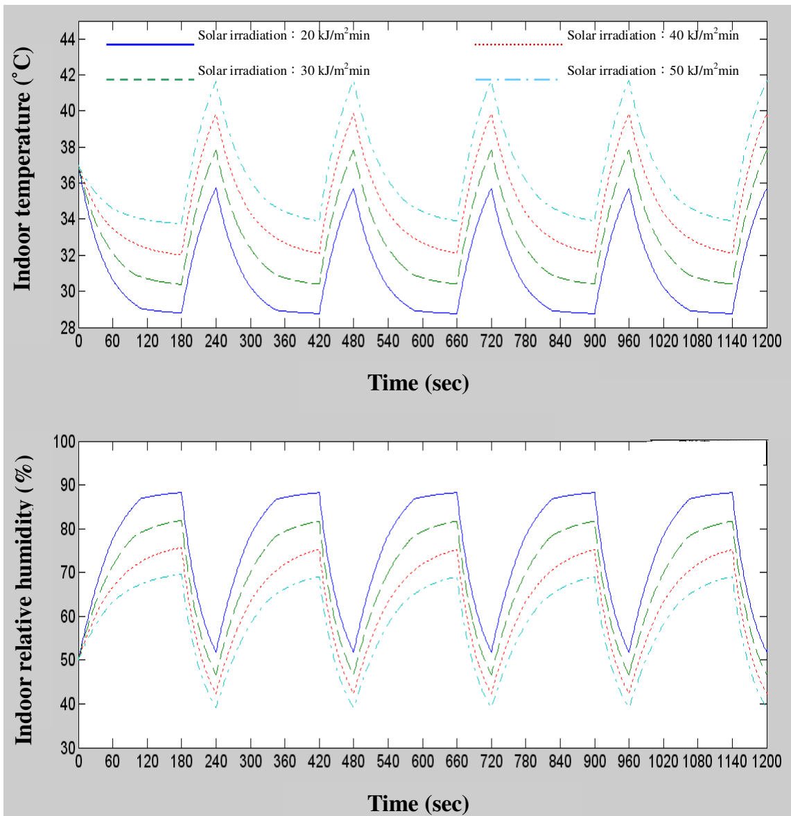
Figure 6. Variation of the inside temperature and relative humidity (fogging on: 3 min and interval: 1 min).
