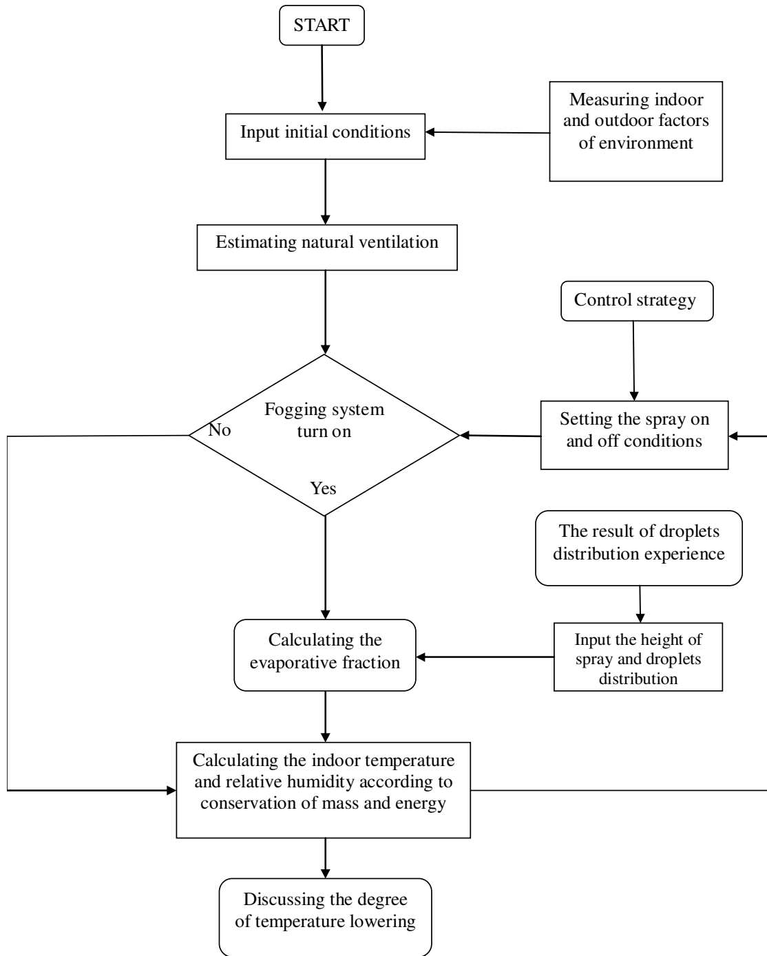
Figure 1. Flowchart showing the simulation procedure.
