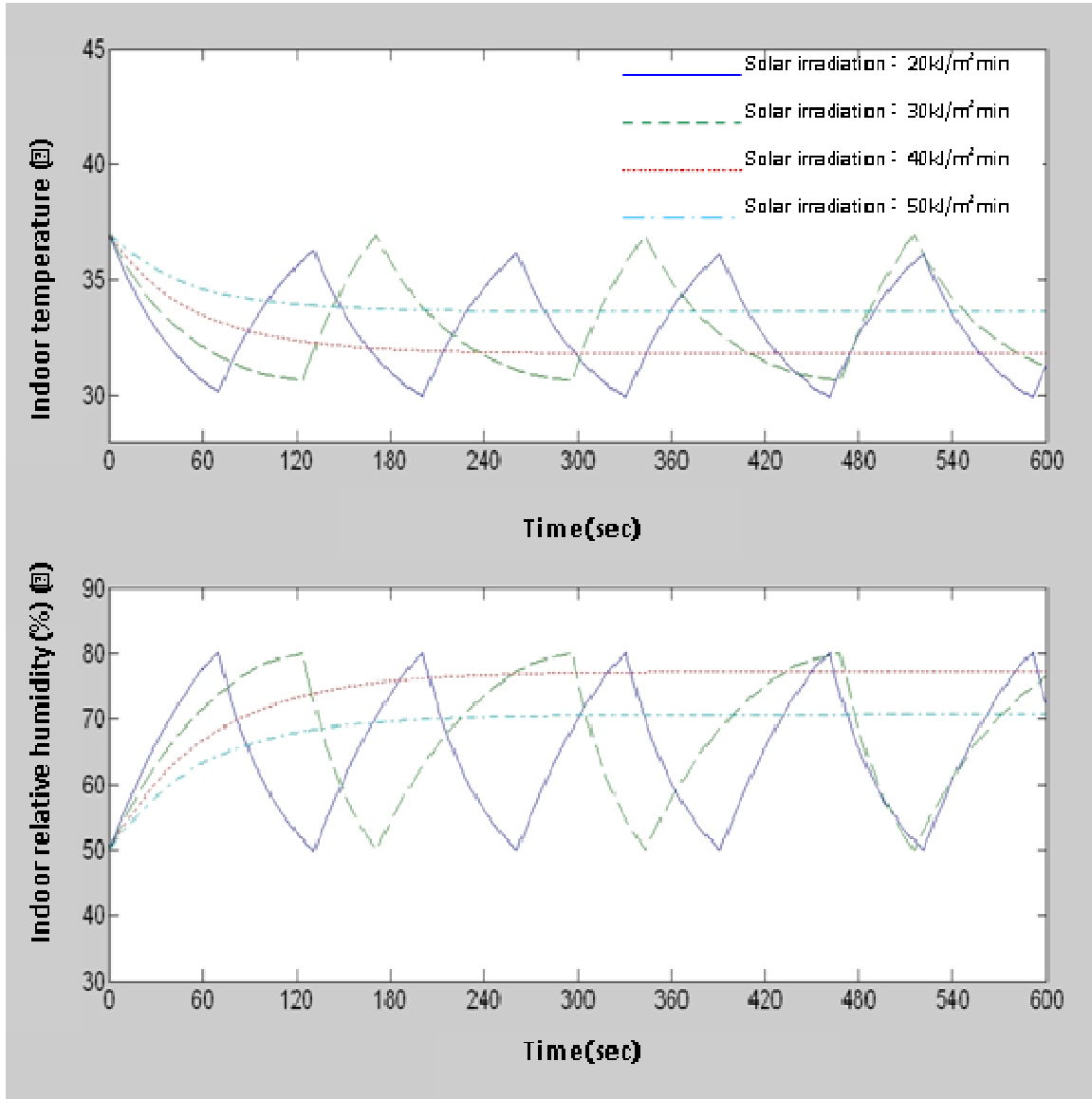
Figure 2. Variation of the inside temperature and relative humidity (fogging on : 50 % RH; off: 80 % RH).
