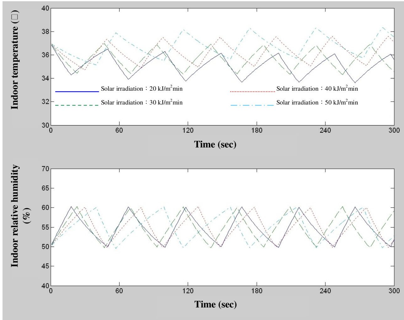
Figure 3. Variation of the inside temperature and relative humidity (spray on: 50 % RH; off: 60 % RH).
