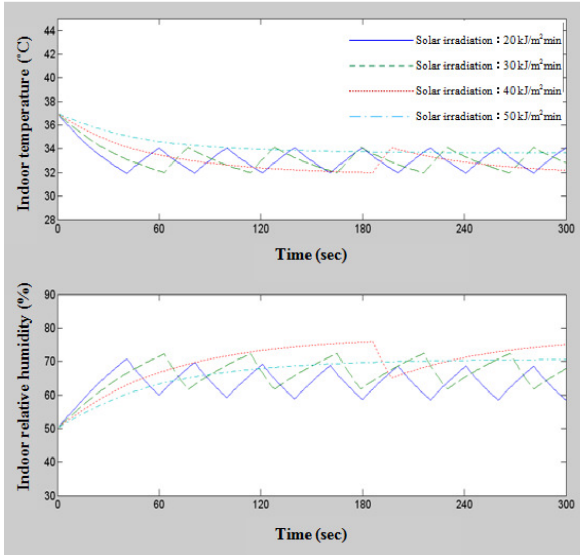
Figure 5. Variation of the inside temperature and relative humidity (spray on: 34°C d.b.; off: 32°C d.b.).
