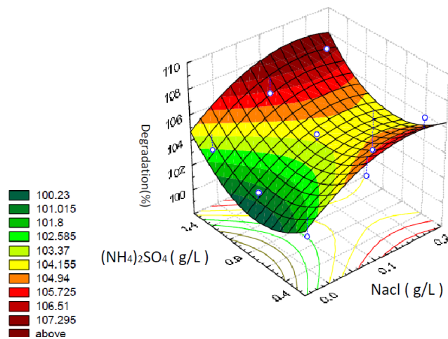
Figure 3. Interaction of (\text{NH}_4)_2\text{SO}_4 (g/l) with NaCl (g/l) with respect to chloroxylenol degradation percentage based on RSM.
