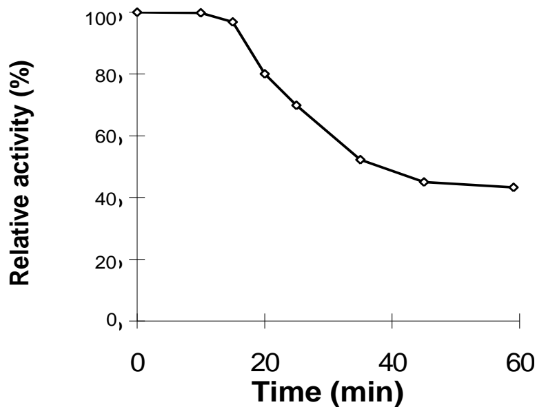
Figure 11. The relative activity of cellulase modified by methanol at different reaction times. The activity of cellulase modified by deionized water as control was defined as 100%.
