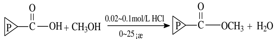
Figure 6. The carboxyl in the side-chain radical of cellulase modified by methanol.
