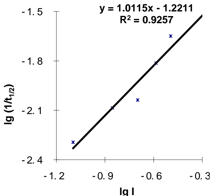
Figure 12. The standard curve plotted with logarithmic of 1/t_{1/2} against logarithmic of concentration of methanol. t_{1/2} and I are the time required for 50% decrease in activity and the concentration of methanol, respectively.
