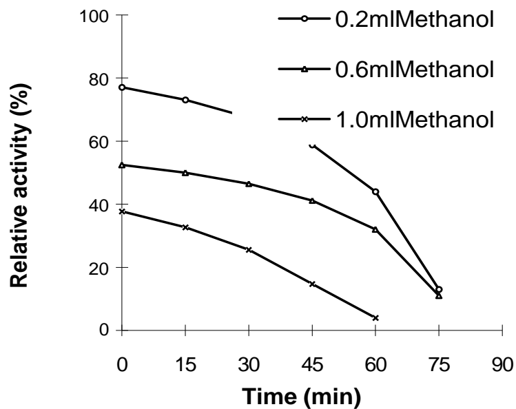
Figure 8. The relative activity of cellulase modified by methanol at different times. The activity of cellulase modified by deionized water as control was defined as 100%.
