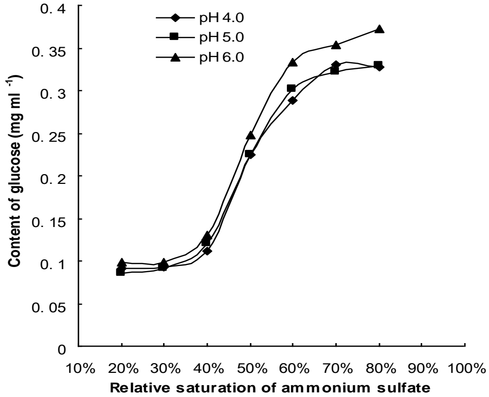
Figure 1. Effect of saturation degree of ammonium sulfate on the activity of cellulase salted out by ammonium sulfate.
