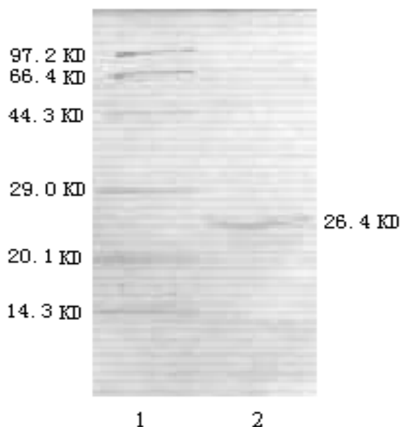
Figure 3. SDS-PAGE analysis of the purification and molecular weight of \beta -endoglucanase. Lane 1, protein markers; lane 2, the purified \beta -endoglucanase.
