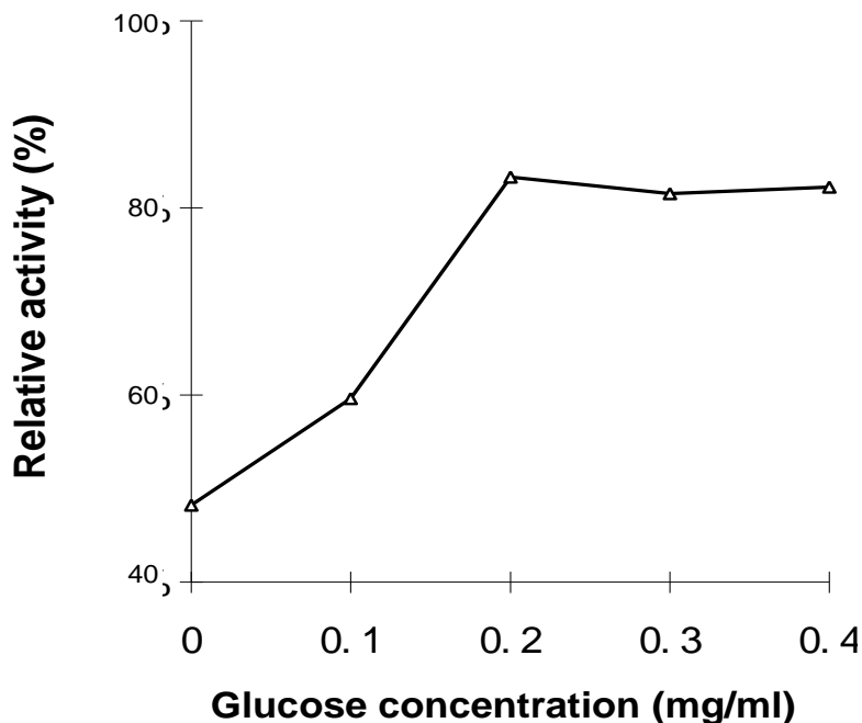
Figure 10. Effect of the concentration of glucose on the relative activity of cellulase modified by methanol. The activity of cellulase using deionized water as control instead of methanol and glucose was defined as 100%.
