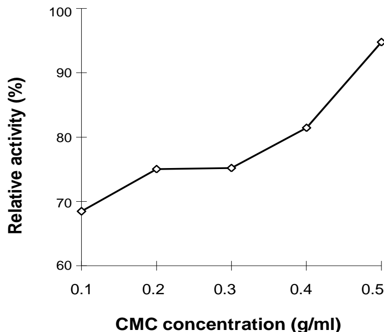
Figure 9. Effect of the concentration of substrate on the relative activity of cellulase modified by methanol. The activity of cellulase using deionized water as control instead of methanol and CMC-Na was defined as 100%.
