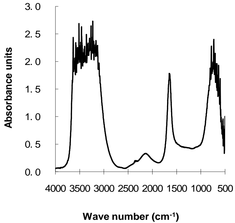
Figure 4. FTIR spectrum of cellulase unmodified.
