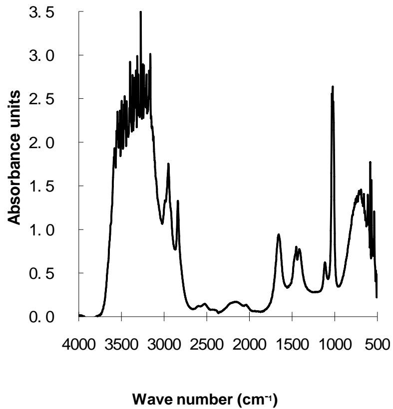
Figure 5. FTIR spectrum of cellulase modified by excess methanol.
