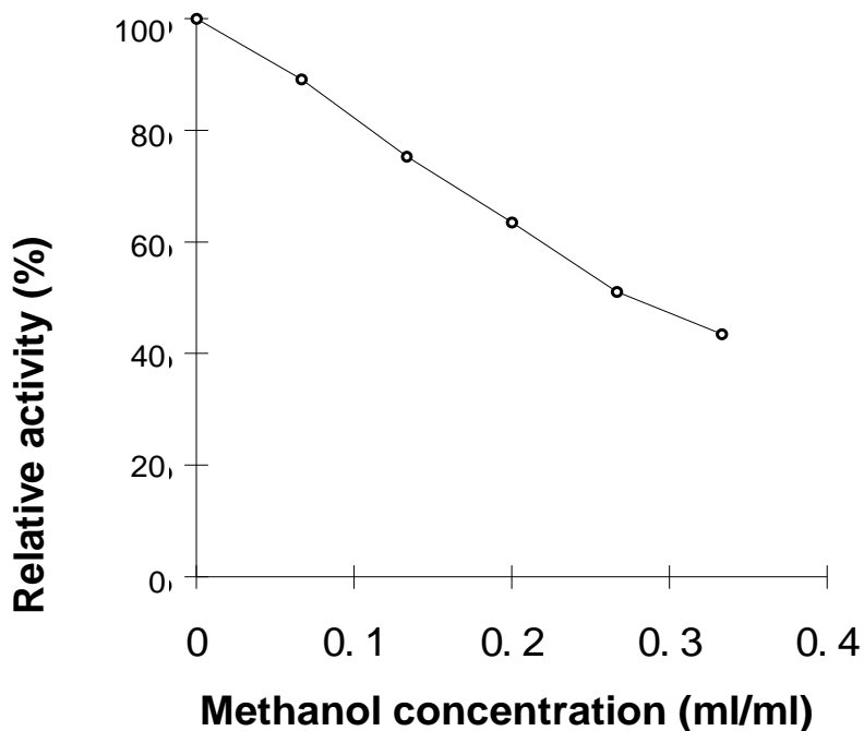
Figure 7. Modification of cellulase with different concentrations of methanol. The activity of cellulase modified by deionized water as control was defined as 100%.
