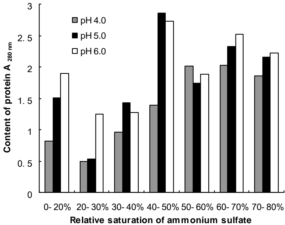
Figure 2. Effect of saturation degree of ammonium sulfate on the content of protein salted out by ammonium sulfate.
