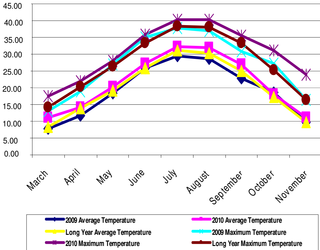
Figure 2. Monthly average and maximum temperature of 2009, 2010 and long term.
