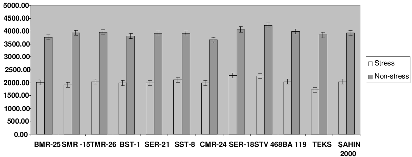
Figure 3. Seed cotton yield (kg ha -1 ) of genotypes under water stress and non stress conditions.
