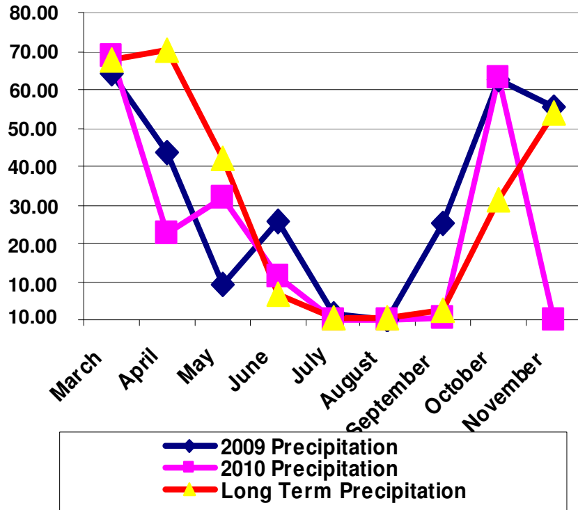
Figure 1. Average precipitation levels (mm) of 2009, 2010 and long term.
