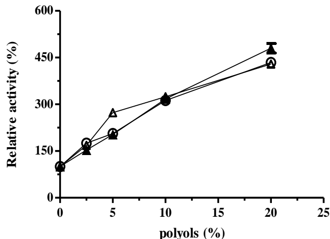
Figure 4. Thermostability of the xylanase at 50°C, with manitol (▲), xylitol (●) and glycerol (△) in different concentrations [2.5 – 20% (w/v)]. Residual activity was assayed after 120 min at 50°C.
