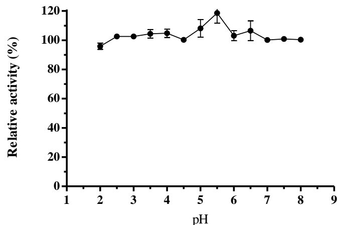
Figure 1. The pH stability of xylanase by A. flavus . The influence of pH on xylanase was verified using McIlvaine buffer 2.0-8.0. Residual activity was assayed after 1 h.
