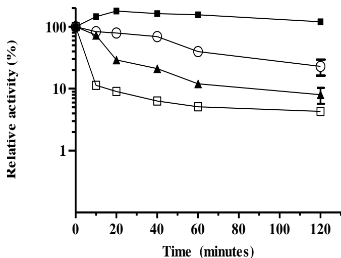
Figure 2. Thermostability of the xylanase of A. flavus . The thermostability was determined using McIlvaine buffer pH 5.0 at 55°C after incubating the enzyme on temperatures of 45 (■), 50 (○), 55 (▲) and 60°C (□). The residual xylanase activity was calculated as the percentage of initial enzyme (before incubation).
