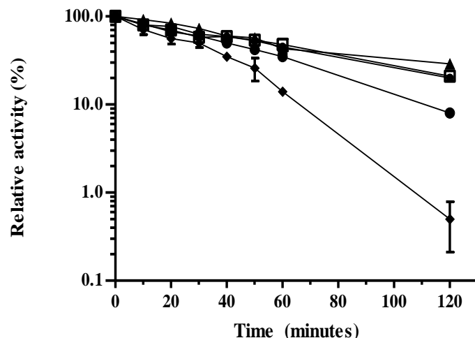
Figure 3. The effect of polyols on thermostability of the xylanase from A. flavus . The enzyme solutions were preincubated at 50°C without the presence of substrate for various times (0 - 120 min) in the presence of glycerol (▲), mannitol (●), xylitol (□) and polyethyleneglycol (◆) at a concentration of 5% prior to enzyme assay at the optimal condition. Control (Δ) without the presence of polyols. The residual xylanase activity was calculated as the percentage of initial enzyme (before incubation).
