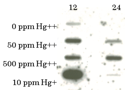
Figure 6. Expression of mercuric reductase ( merA ) gene in water microcosms inoculated with P. stutzeri under various concentrations of mercuric ions following 12 and 24 hours of exposure.
