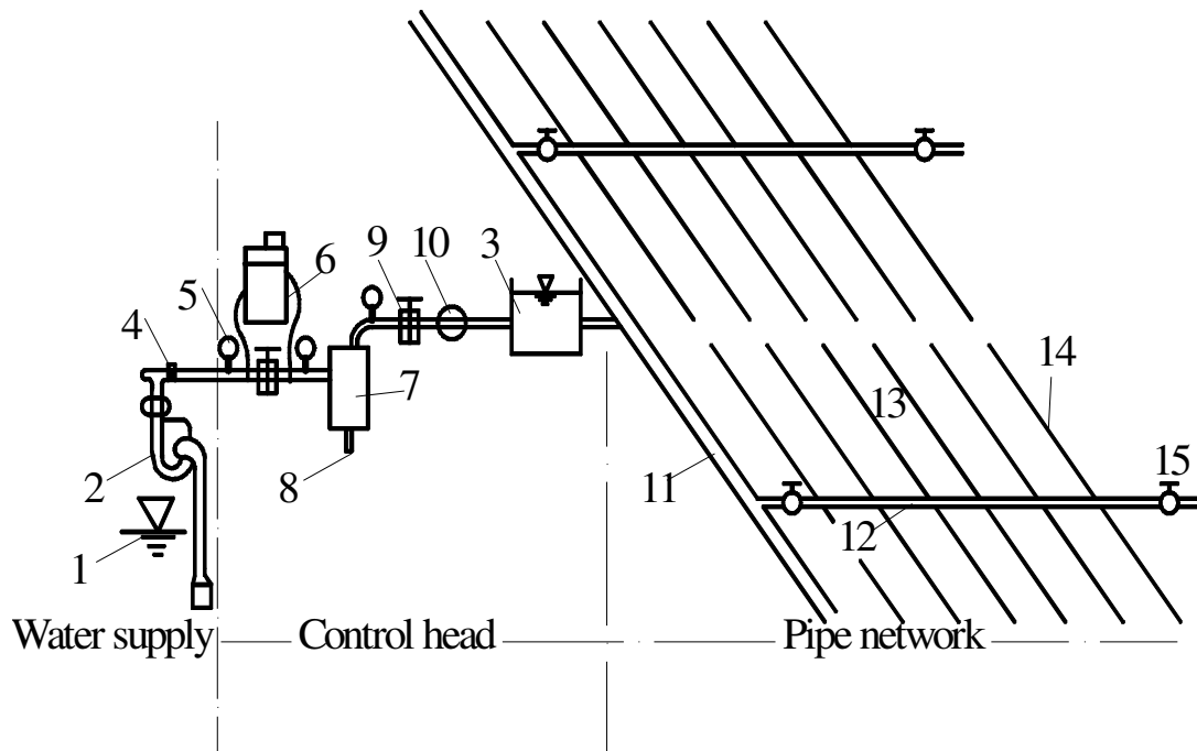
Figure 1. Micro-pressure drip system components. 1 = pump; 2 = water supply; 3 = pressure regulator; 4 = back-flow prevention valve; 5 = pressure valve; 6 = fertilizer injecting device; 7 = filter; 8 = waste-drain valve; 9 = valve; 10 = flow meter; 11 = mainlines; 12 = manifolds; 13 = laterals; 14 = emitters; 15 = flush-out valve.
