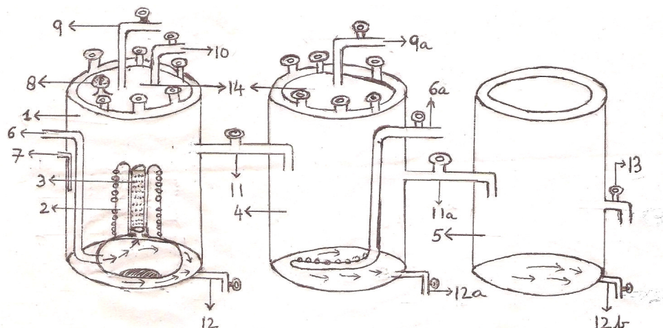
Figure 1. Schematic representation of multistage continuous fermentor (1, unit A ; 2, unit B ; 3, unit C ; 4, unit D ; 5, unit E ; 6, aeration unit ; 6a, aeration unit ; 7, thermostatic heating device ; 8, pressure gauge ; 9, exhaust ; 9a, exhaust ; 10, extra port for medium inlet ; 11, connecting pipe with regulator ; 11a, connecting pipe with regulator ; 12, outlet for dead yeast cells and washing ; 12a, outlet for dead yeast cells and washing ; 13, drain pipe for pullulan outlet ; 14, replaceable lid).
