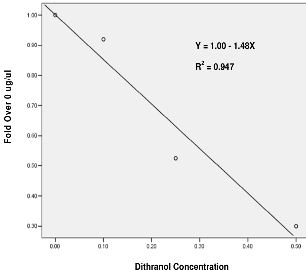
Figure 2. Pearson's correlation between normalized EGF receptor expression levels in HaCaT cells and concentrations of dithranol for treatment.
