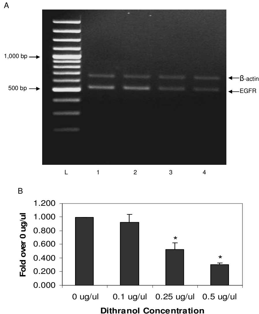
Figure 1. RT-PCR analysis of EGFR expression in HaCaT cells treated with increasing dithranol concentrations (0, 0.1, 0.25 and 0.5 ug/ml) for 4 h. (A) 2% agarose gel electrophoresis showing mRNA transcripts of EGFR and \beta -actin. Lane L: 100-bp DNA ladders, whereas lanes 1 to 4 corresponding to increasing dithranol concentrations used for treating HaCaT cells. (B) Average fold over expression at 0 ug/ml dithranol. A symbol, *, indicating a statistically significant difference ( P < 0.05 ).
