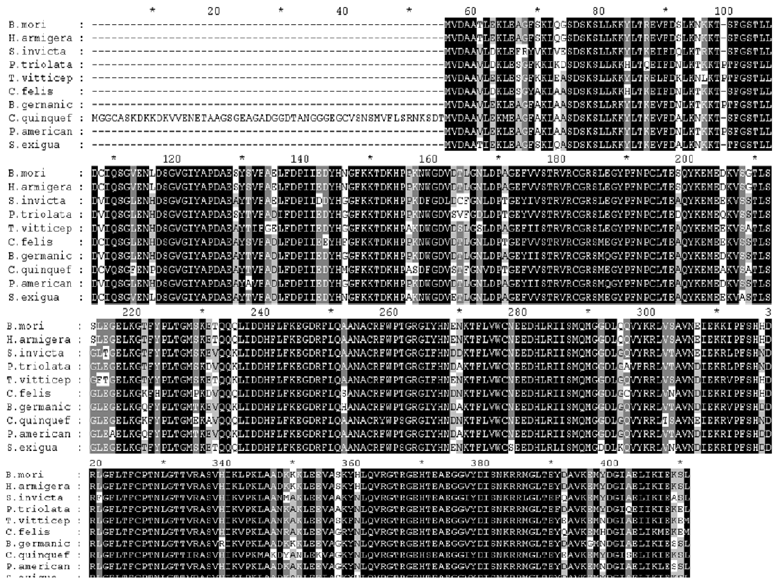
Figure 2. Multiple sequence alignment of amino acids of Bombyx mori AK and AKs from other insects. The identical amino acids were shown in black shade and the conserved amino acids were shown in gray shade. The aligned AKs were from B. mori (GenBank accession No. NP_001037402.1), H. armigera (ABU98622.1), S. exigua (ACU68932.1), P. americana (AAT77152.1), T. vitticeps (ABJ88949.1), C. felis (CAZ65719.1), S. invicta (ACF04198.1), P. striolata (ABZ10961.1), B. germanica (ABC86902.1) and C. quinquefasciatus (XP001849654.1)
