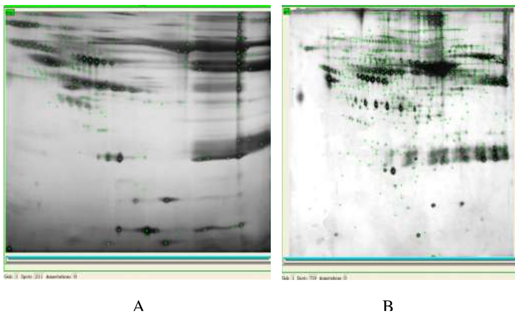
Figure 3. Comparison of 2-DE gel images of human serum proteins in IPG (pH 4-7 and 18 cm) via sample in-cup (A) and sample in-gel (B) application and analyzed with Image master 2D platinum 6.0.
