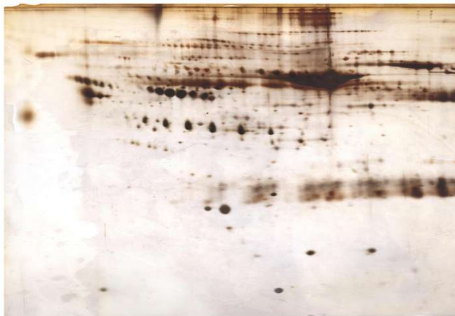
Figure 2. Two-dimensional pattern of human serum proteins in IPG (pH 4-7 and 18 cm) via sample in gel application, stained with silver.
