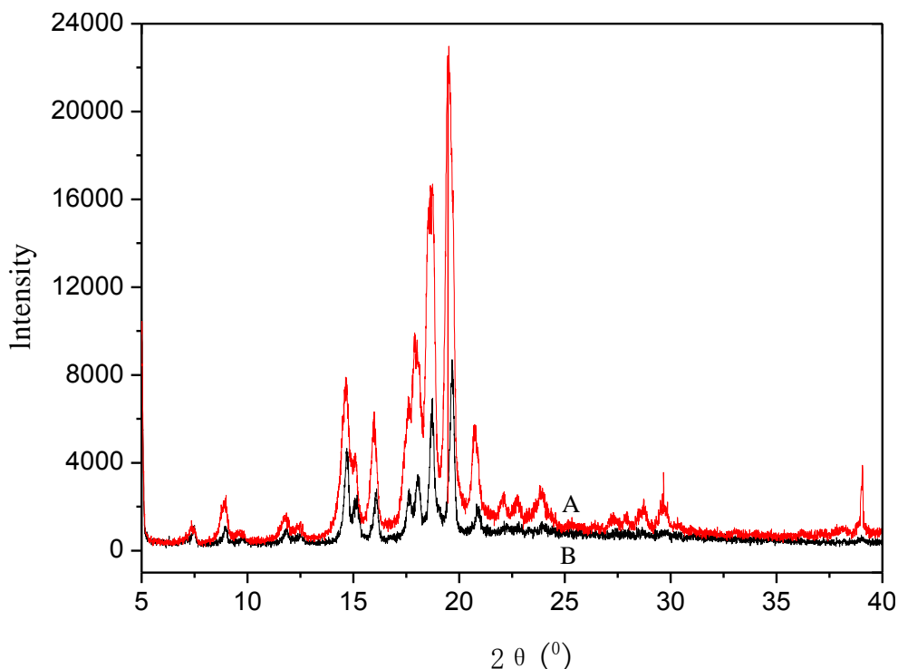
Figure 4. X-ray diffraction patterns of the ergosterol crystal. The powder X-ray diffraction (XRD) patterns were recorded on a PW1700 wide Angle X-ray diffractometer with Cu K \alpha radiation ( \lambda=1.54184 Å) operated at 40 kV and 30 mA. The scanning speed was 0.02^\circ \text{ min}^{-1} in the 2\theta range from 0.50 to 40.00^\circ . A, Standard sample of ergosterol; B, the ergosterol produced by corn straw.
