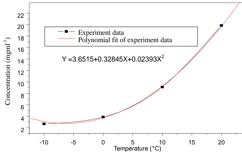
Figure 1. Solubility curve of ergosterol crystal temperature.
