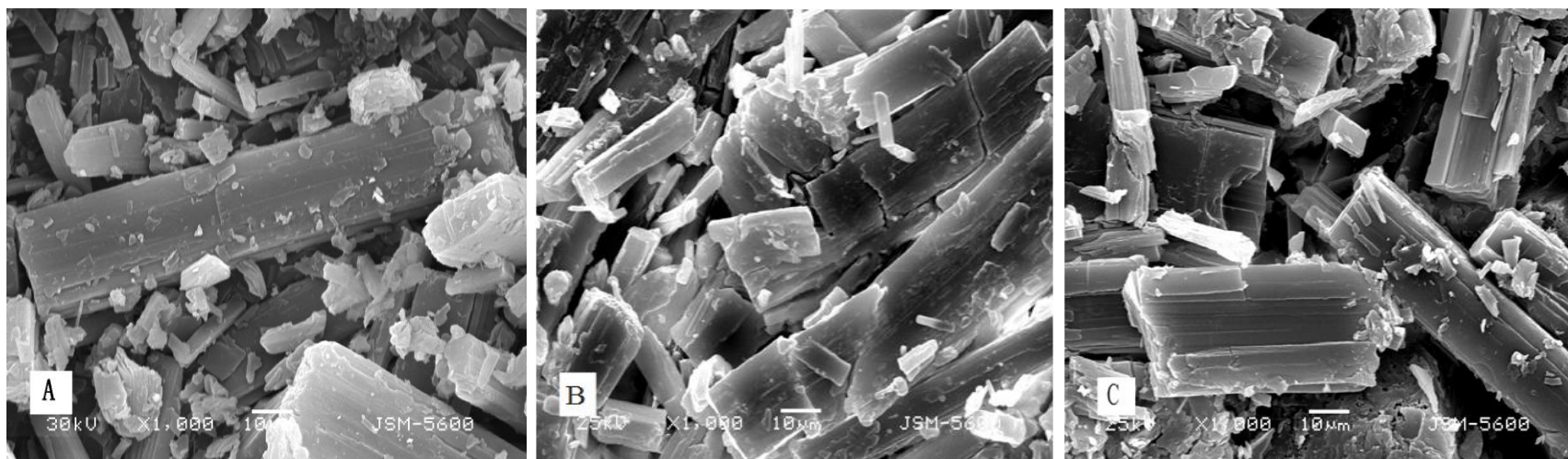
Figure 2. The SEM images of ergosterol. (A) The SEM image of ergosterol standard sample. (B) The SEM image of product with TD. (C) The SEM image of product with CT. SEM, Scanning electron microscope; CT, constant temperature; TD, temperature drop.
