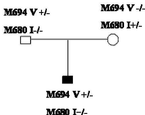
Figure 1. Pedigree illustrating mode of mutation inheritance. Open boxes are related to parents that is asymptomatic FMF gene carrier, black box is related to child with FMF due to M694V/M680I compound heterozygote mutation.
