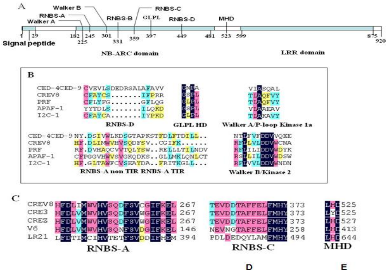
Figure 5. A. Conserved motifs of the NB-ARC domain in CreV8 . Ced-4 / CED-9 , PRF , APAF-1 and I2C-1 are R genes that contain NB-ARC domains. Seven conserved motifs are labeled with their names under the corresponding positions (marked by black lines). Numbers indicate the distance from the protein termini to the proximal and distal aligned blocks, and the distances between the blocks. B. Gene structure of CreV8 , showing the position of each motif. C. Alignments of RNBS-A motifs of CreV8 , Cre3 , CreZ , V6 and Lr21 . D. Alignment of RNBS-C motif of CreV8 , Cre3 , CreZ , V6 and Lr21 . E. Alignment of the MHD motifs of CreV8 , Cre3 , CreZ , V6 and Lr21 .
