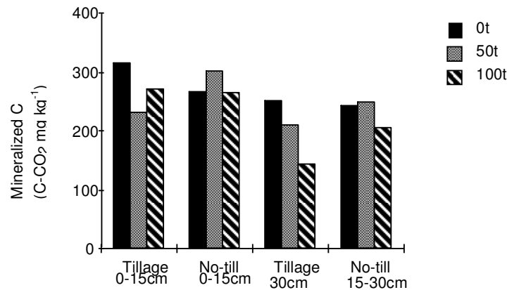
Figure 2. Effect of tillage and liquid manure on cumulative C mineralized over 270 d incubation.
