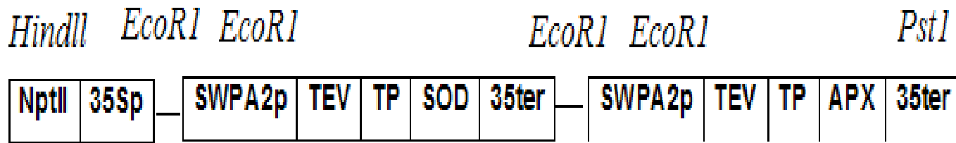
Figure 1. The SSA mode of expression vector in modified genetic potato introduced by CuZnSOD and APX genes.
