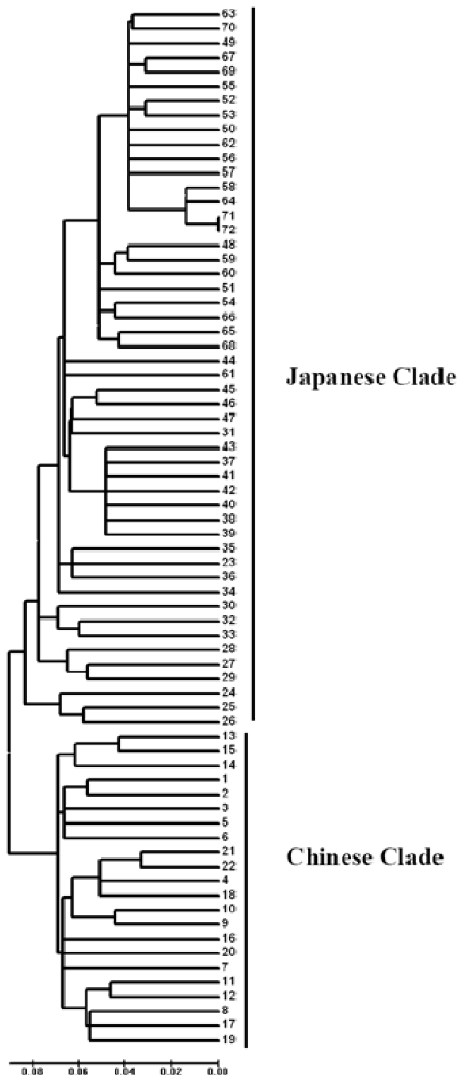
Figure 4. UPGMA tree of all individuals based on the Nei and Li (1979) distance (1-9: A170; 10-22: B21; 23-46: Ariake Sea; 47-70: Ise Bay).
