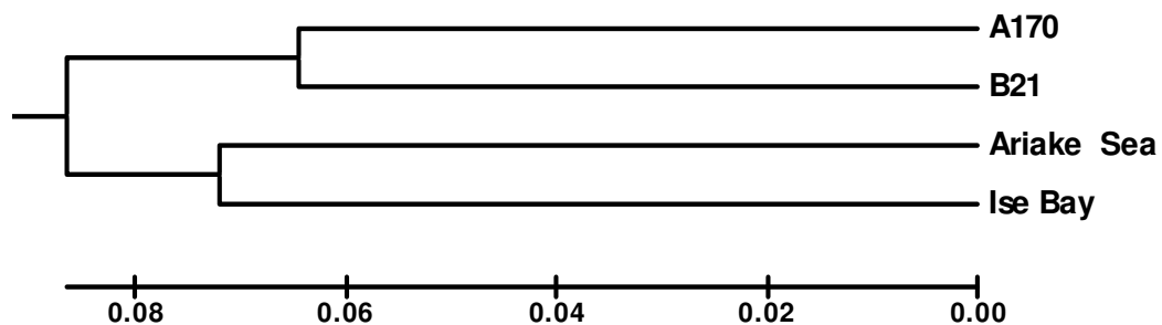
Figure 3. The UPGMA tree based on the Nei's genetic distances.
