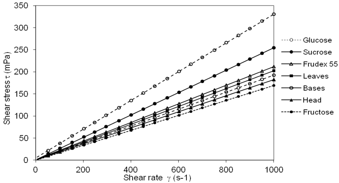
Figure 2. Shear stress vs. shear rate of the different syrups at 70°Brix and 25°C.
