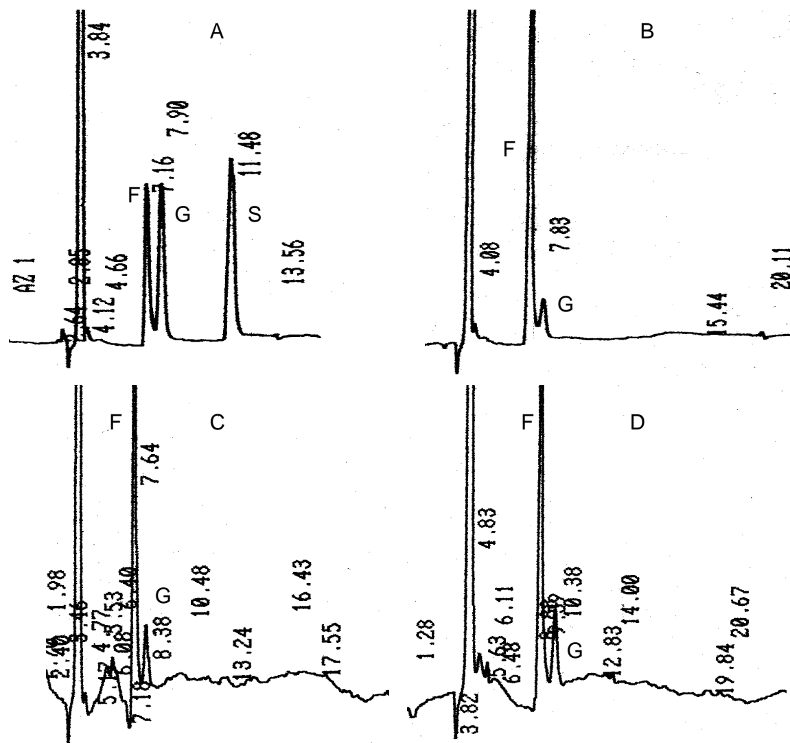
Figure 1. HPLC spectra of: A, Standards of fructose (F), glucose (G) and sucrose (S); B, Agave head syrup; C, Agave bases syrup; D, Agave leaves syrup.
