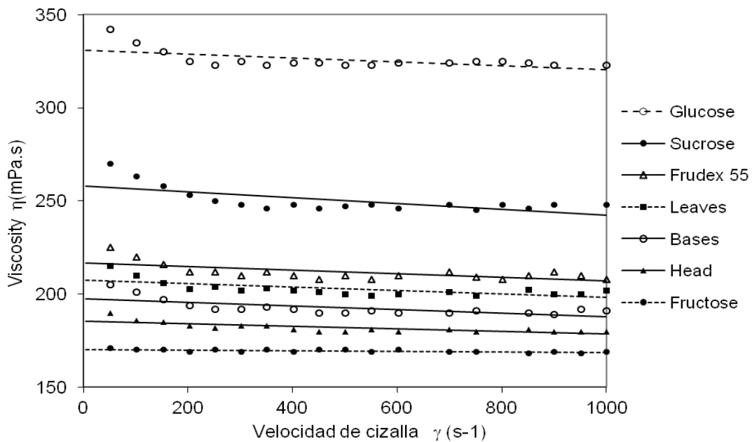
Figure 3. Viscosity vs. shear rate of the different syrups at 70°Brix and 25°C.
