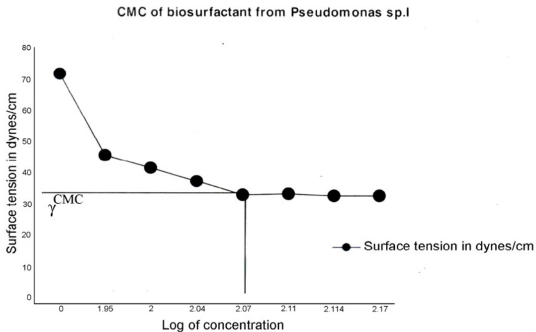
Figure 2. CMC of biosurfactant from Pseudomonas sp. I.
