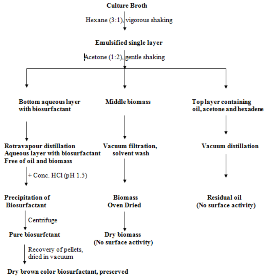
Figure 1. Scheme for extraction of biosurfactant from culture broth
