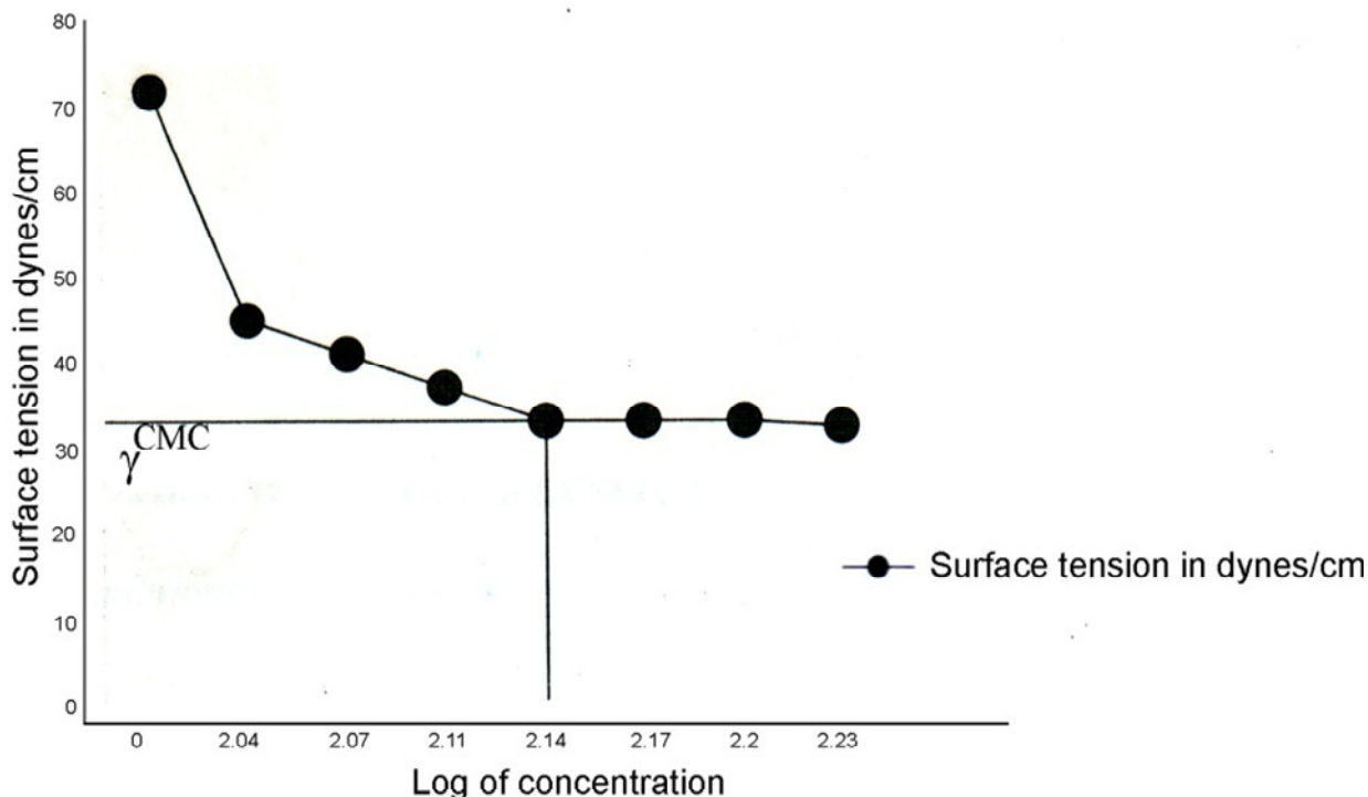
Figure 3. CMC of biosurfactant from Pseudomonas sp. II.
