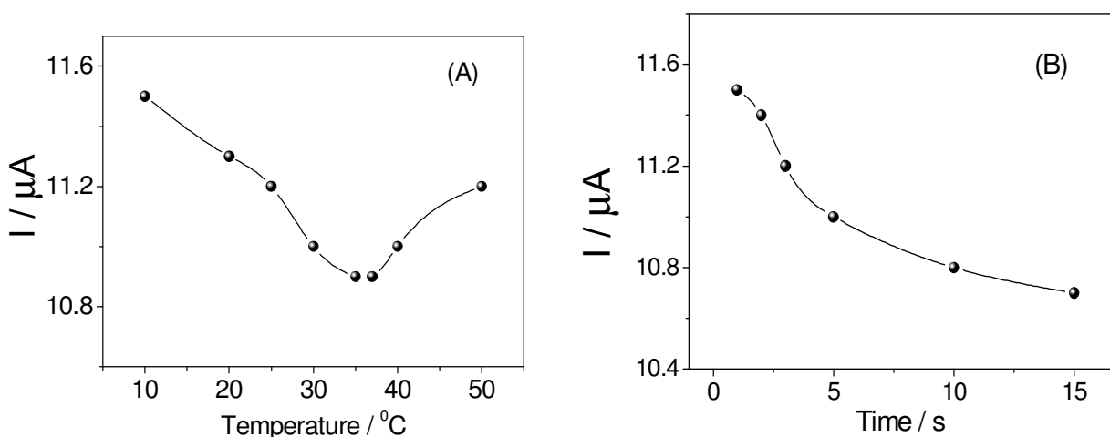
Figure 4. Effect of incubation temperature (A) and incubation time (B) on CV oxidation peak current in pH 7.0 PBS solution.
