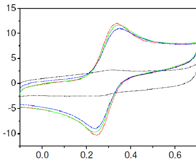
Figure 2. Cyclic voltammograms of different electrodes in PBS (pH = 7.0) at a scan rate of 50 mV/s. (a) bare gold electrode, (b) anti-AFP-Fc/nano-Au/MWCNTs/CS composite membrane modified electrode, (c) the modified electrode blocked with BSA and (d) the immunosensor incubated with 10 ng/ml AFP.
