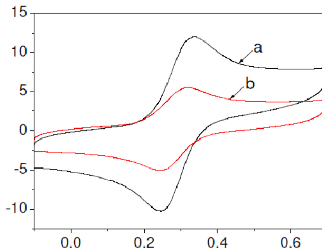
Figure 3. CVs of different electrodes constructed with anti-AFP-Fc/nano-Au/MWCNTs/CS composite membrane (a) and anti-AFP-Fc/nano-Au/CS composite membrane (b).
