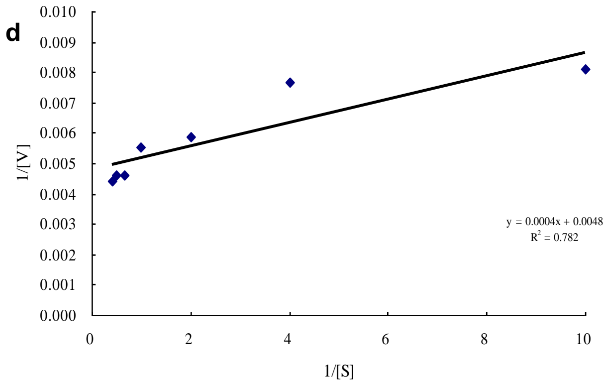
Figure 4. Lineweaver–(a), Burk plots of PPO for catechol, (b), POD for guaiacol, (c) APX for ascorbic acid and (d), H 2 O 2 .
