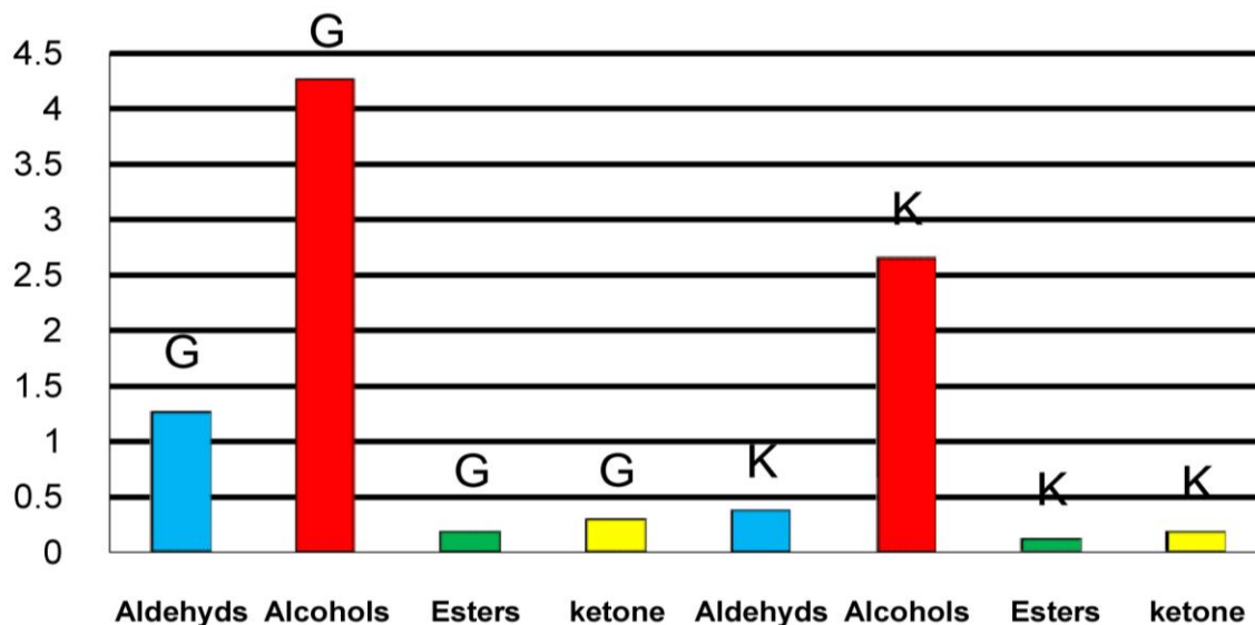
Figure 2. Comparison of oxygenated compounds (%) - aldehydes, alcohols, esters and ketones of Paizeh figs located in two different regions, Garmsar (G) and Karaj (K).
