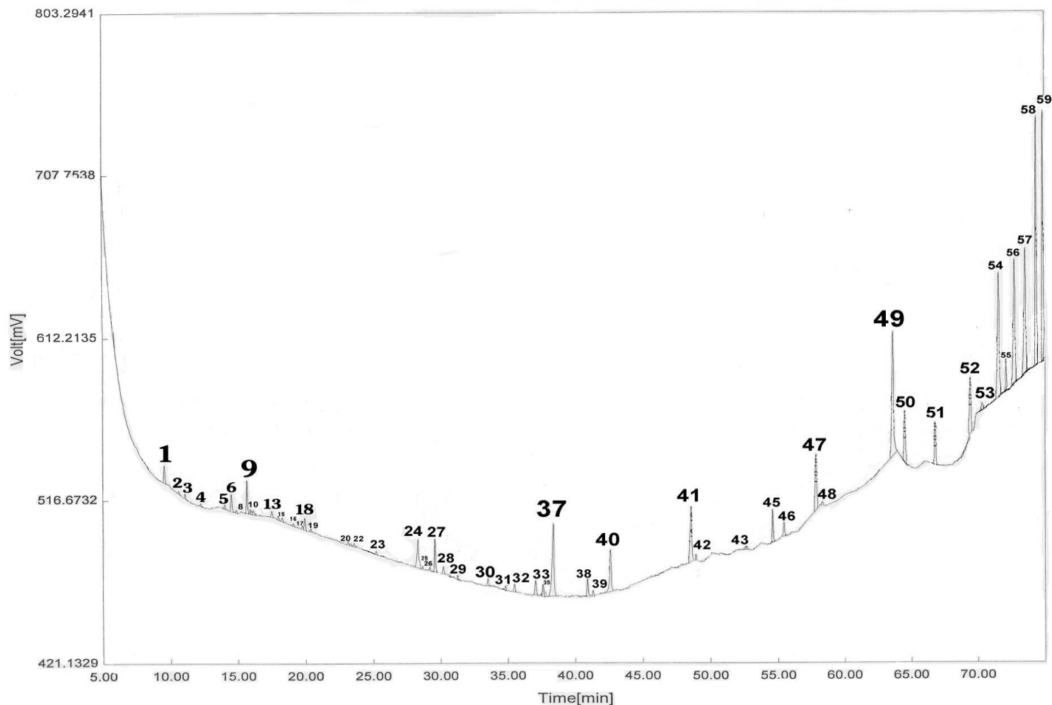
Figure 1. HRGC chromatogram of Ficus carica fruit volatile compounds.
