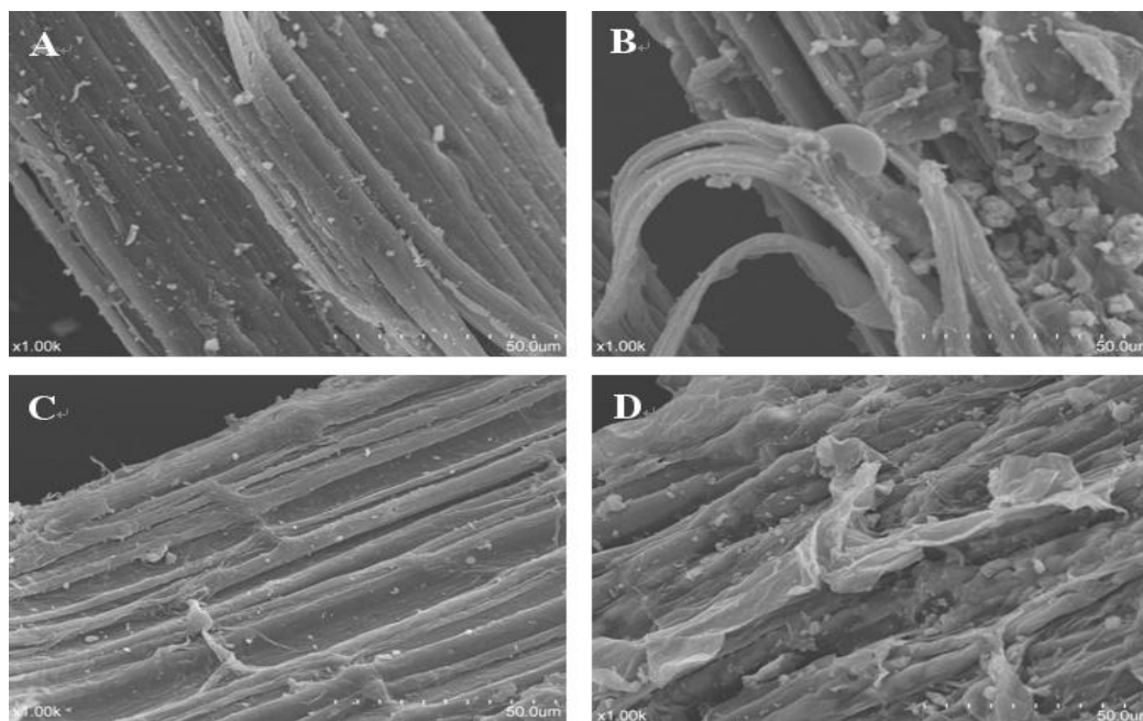
Figure 5. SEM of rice straw and corn stalk samples. Rice straw before enzymatic hydrolysis (A), corn stalk before enzymatic hydrolysis (B); rice straw after enzymatic hydrolysis (C) and corn stalk (D). SignalName=SE, accelerating voltage=20000 volt, Deceleration voltage=0 v, Magnification=1000, working resistance=9400 um, Emission current=50000 nA.
