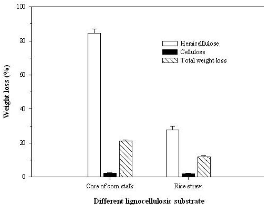
Figure 4. Degradation of lignocellulosic components of different substrates in enzymatic hydrolysis process.
